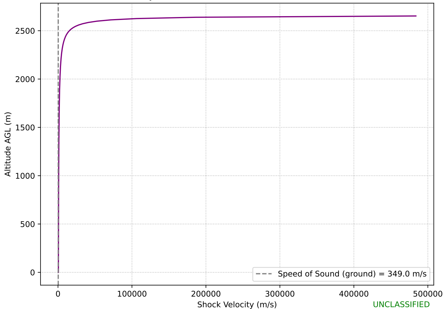
Shock Velocity Profile for 2250.000 kt at HOB=2666.0 m (Weak)
