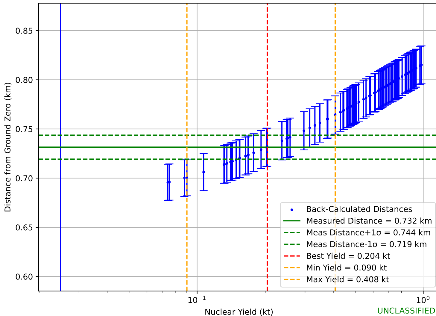
Back-Calculated Distance vs Nuclear Yield Plot
