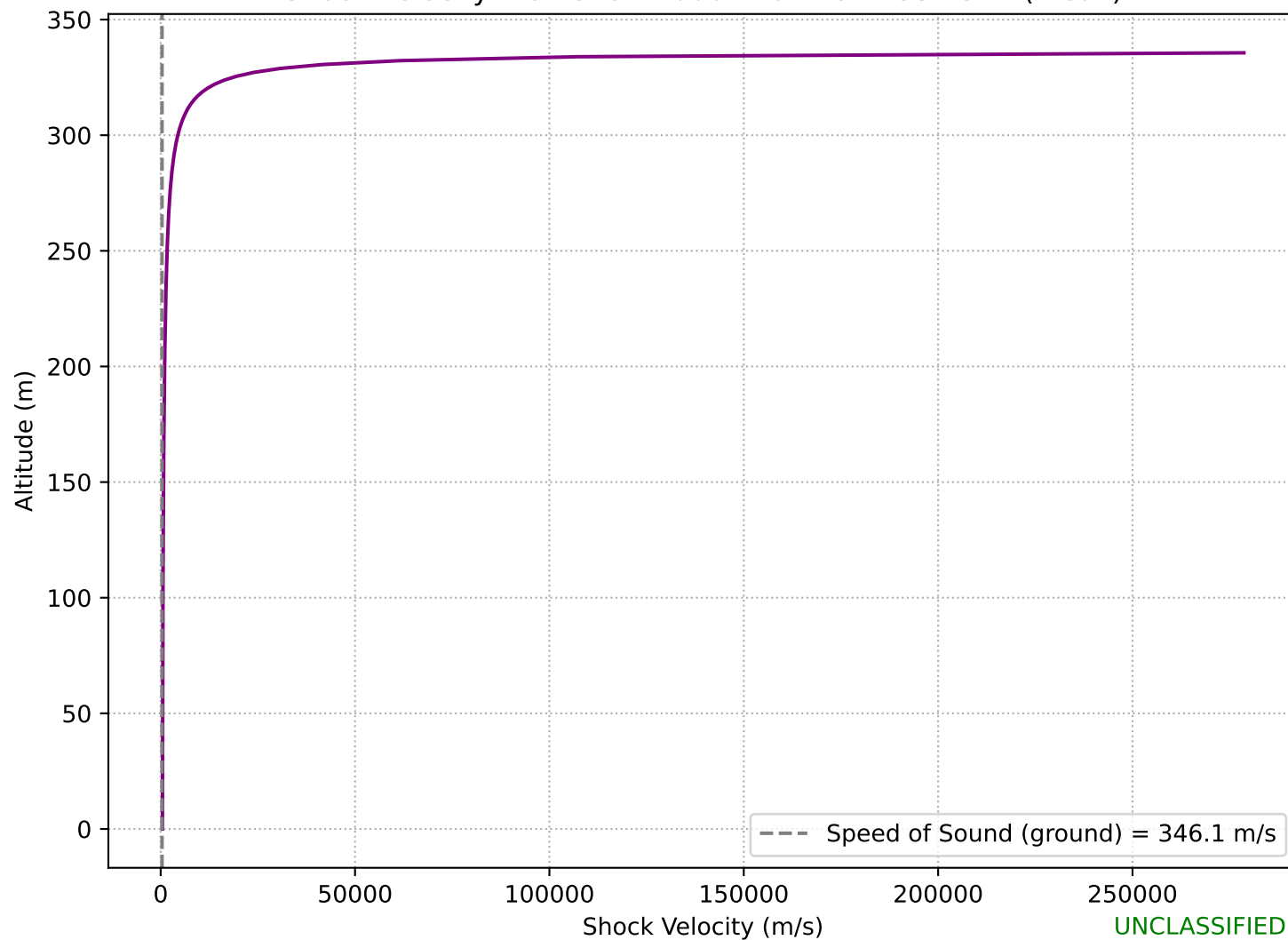
Shock Velocity Profile for 2.000 kt at HOB=337.3 m (Weak)
