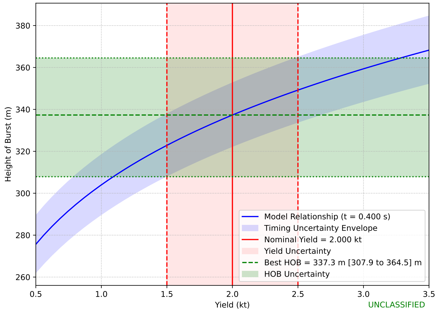
Calculated HOB vs. Yield (Weak Shock Model)
