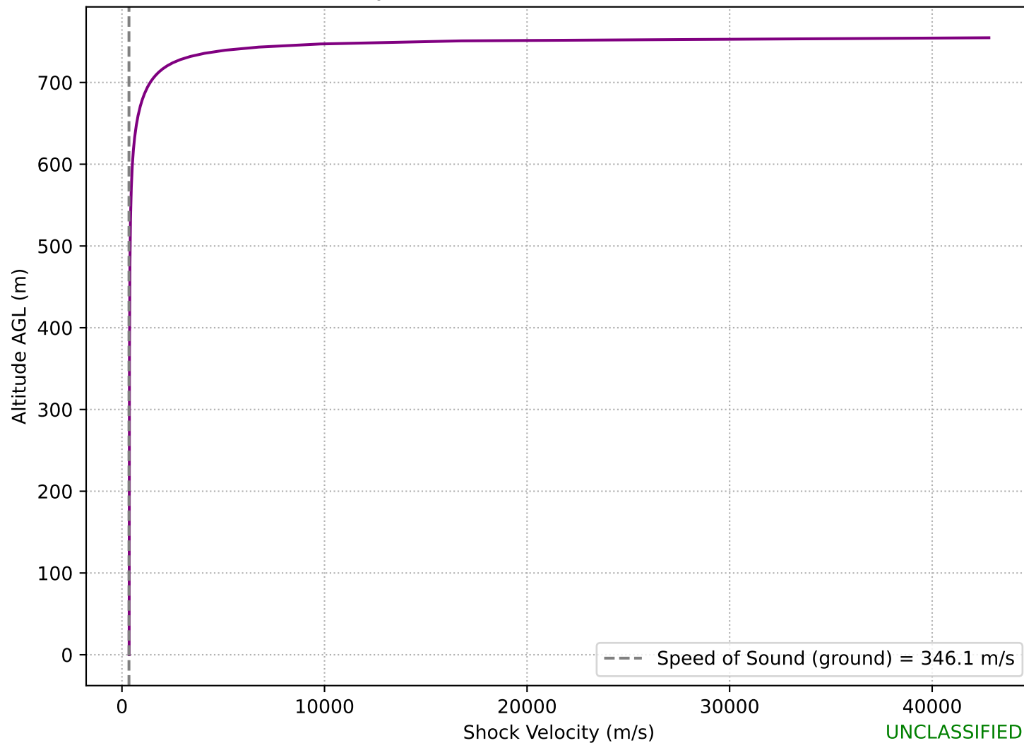
Shock Velocity Profile for 0.250 kt at HOB=758.5 m (Weak)
