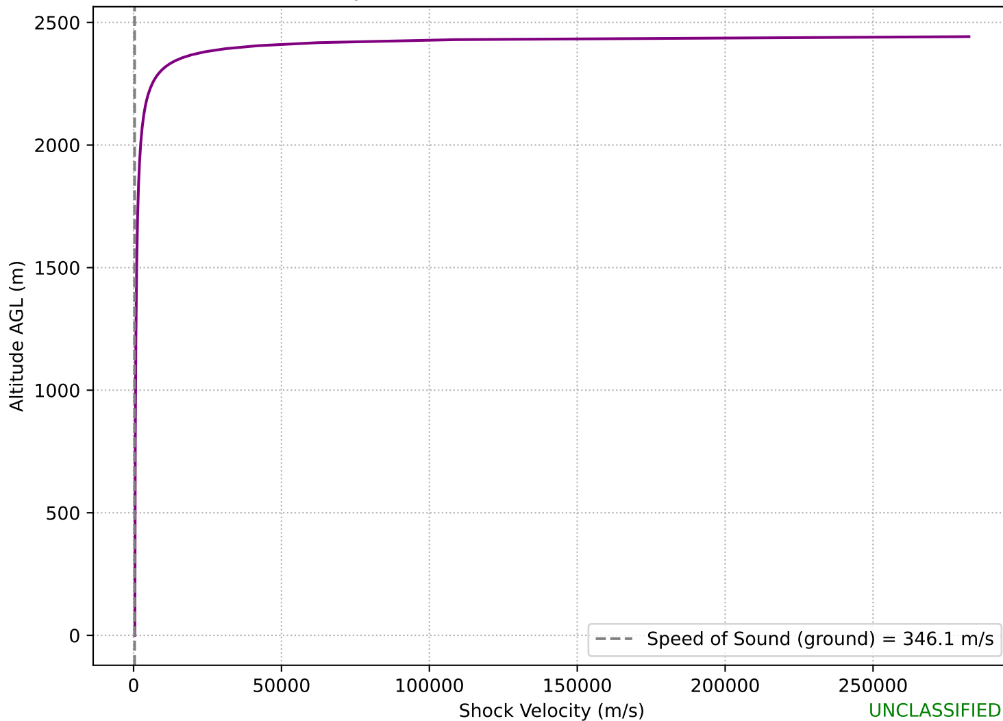
Shock Velocity Profile for 500.000 kt at HOB=2454.5 m (Weak)
