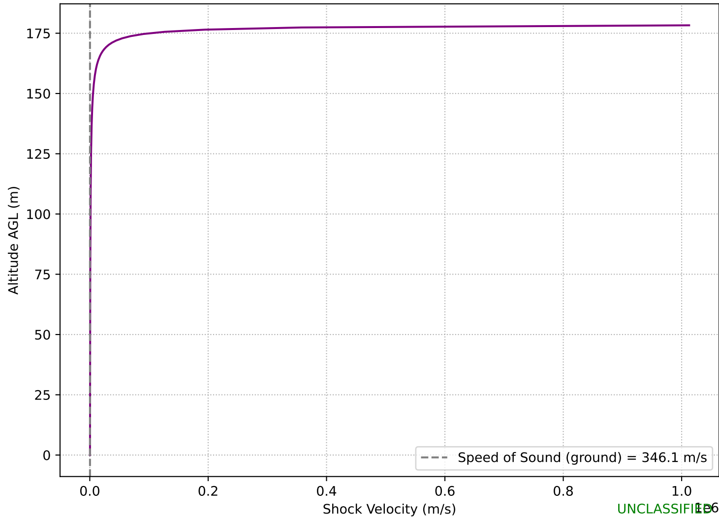
Shock Velocity Profile for 1.300 kt at HOB=179.2 m (Strong)
