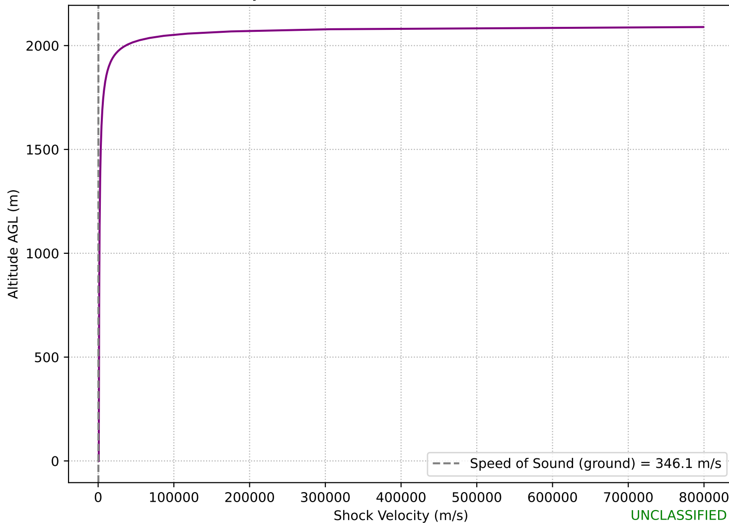
Shock Velocity Profile for 4000.000 kt at HOB=2099.9 m (Weak)
