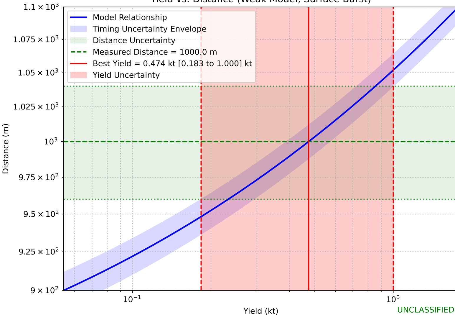
Yield vs. Distance (Weak Model, Surface Burst)
