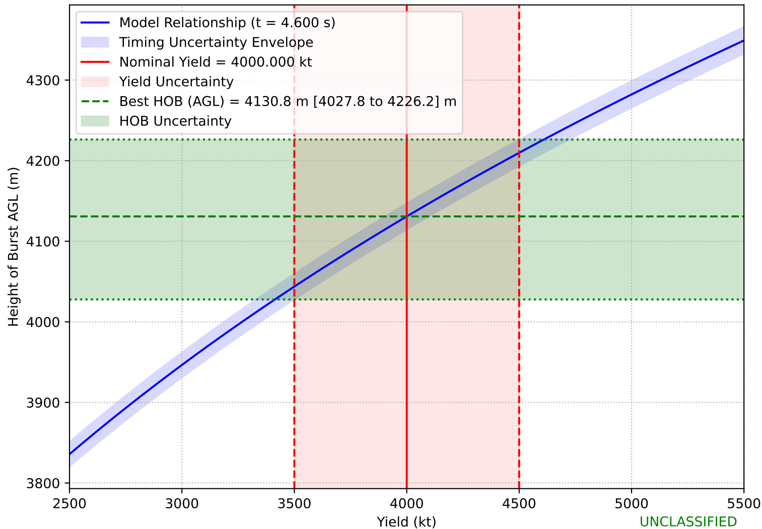
Calculated HOB vs. Yield (Weak Shock Model)
