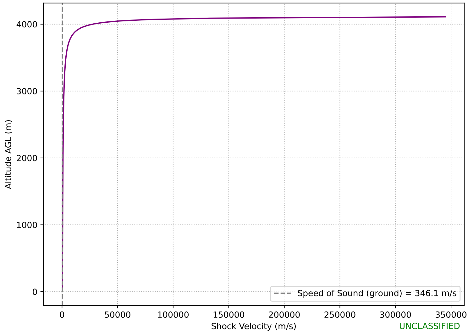
Shock Velocity Profile for 4000.000 kt at HOB=4130.8 m (Weak)
