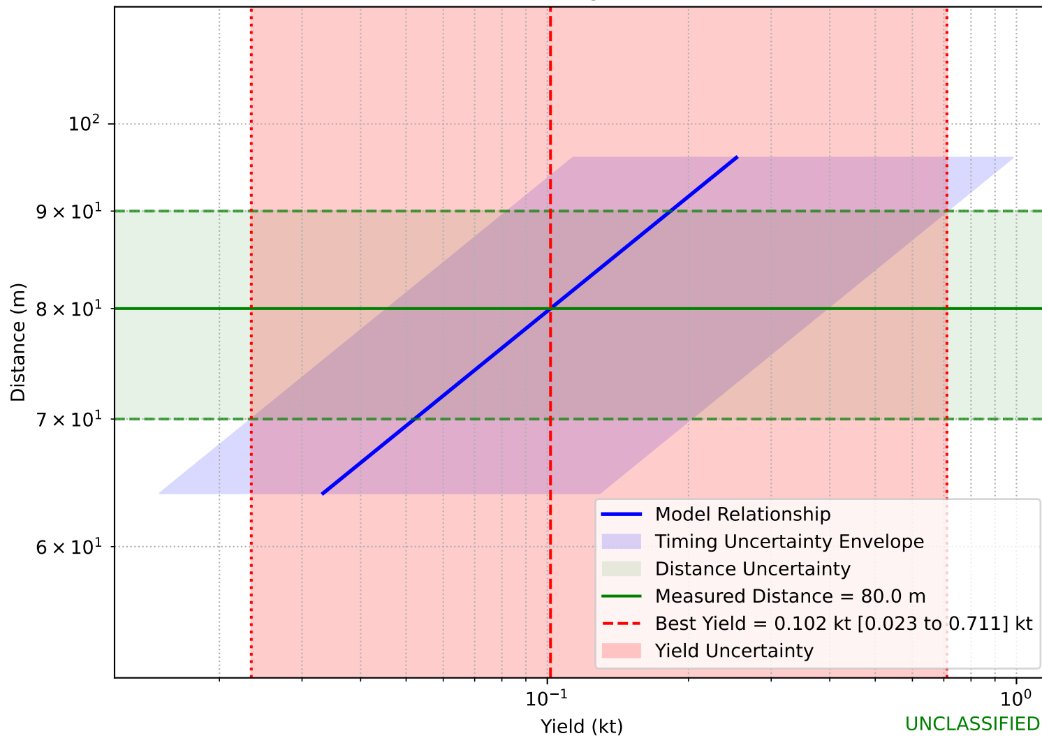
Yield vs. Distance (Strong Model, Surface Burst)
