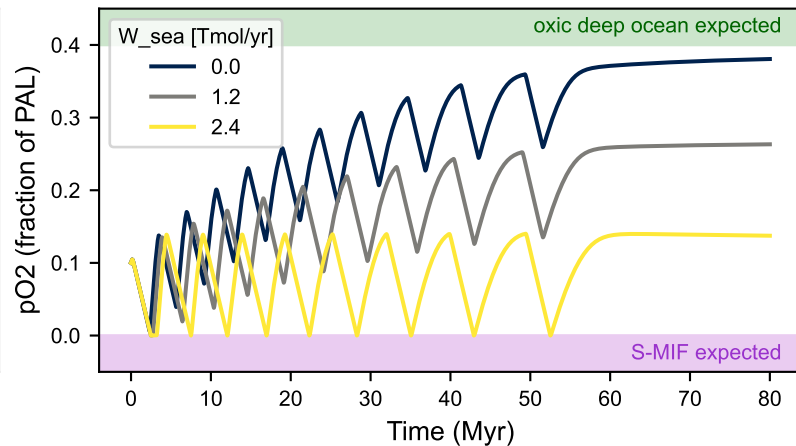
Seafloor weathering [Tmol/yr]
