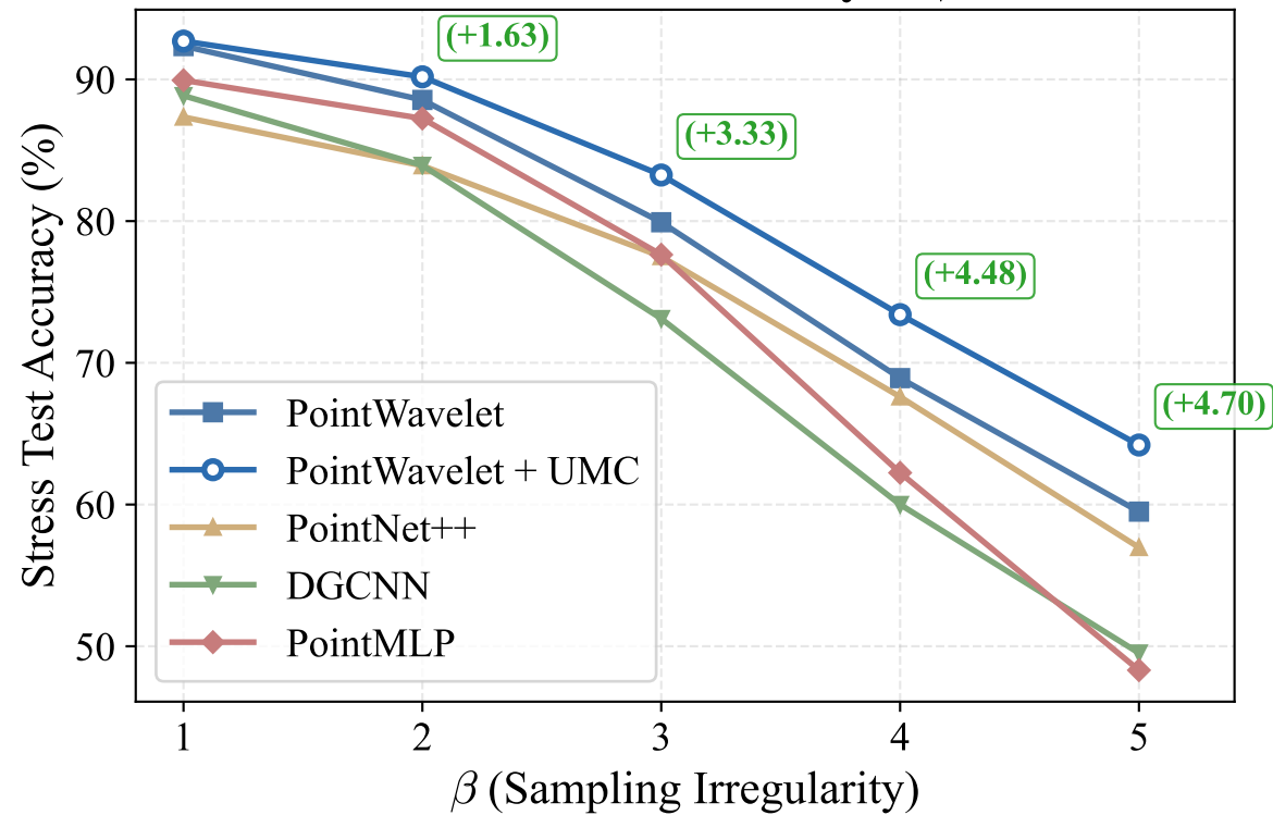
Stress Test Accuracy vs \beta
