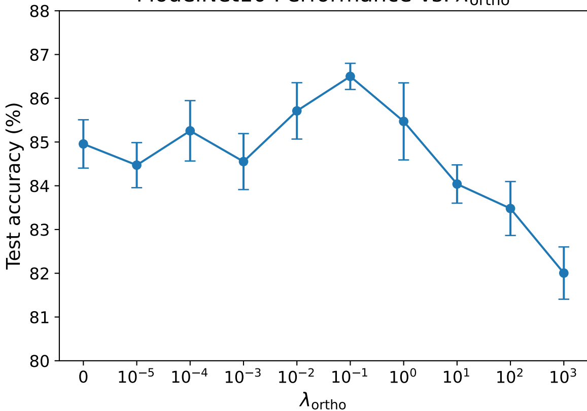
ModelNet10 Performance vs. \lambda_{\text{ortho}}
