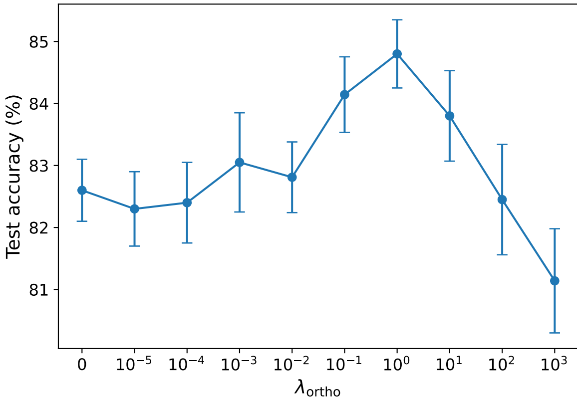
ModelNet40 Performance vs. \lambda_{\text{ortho}}
