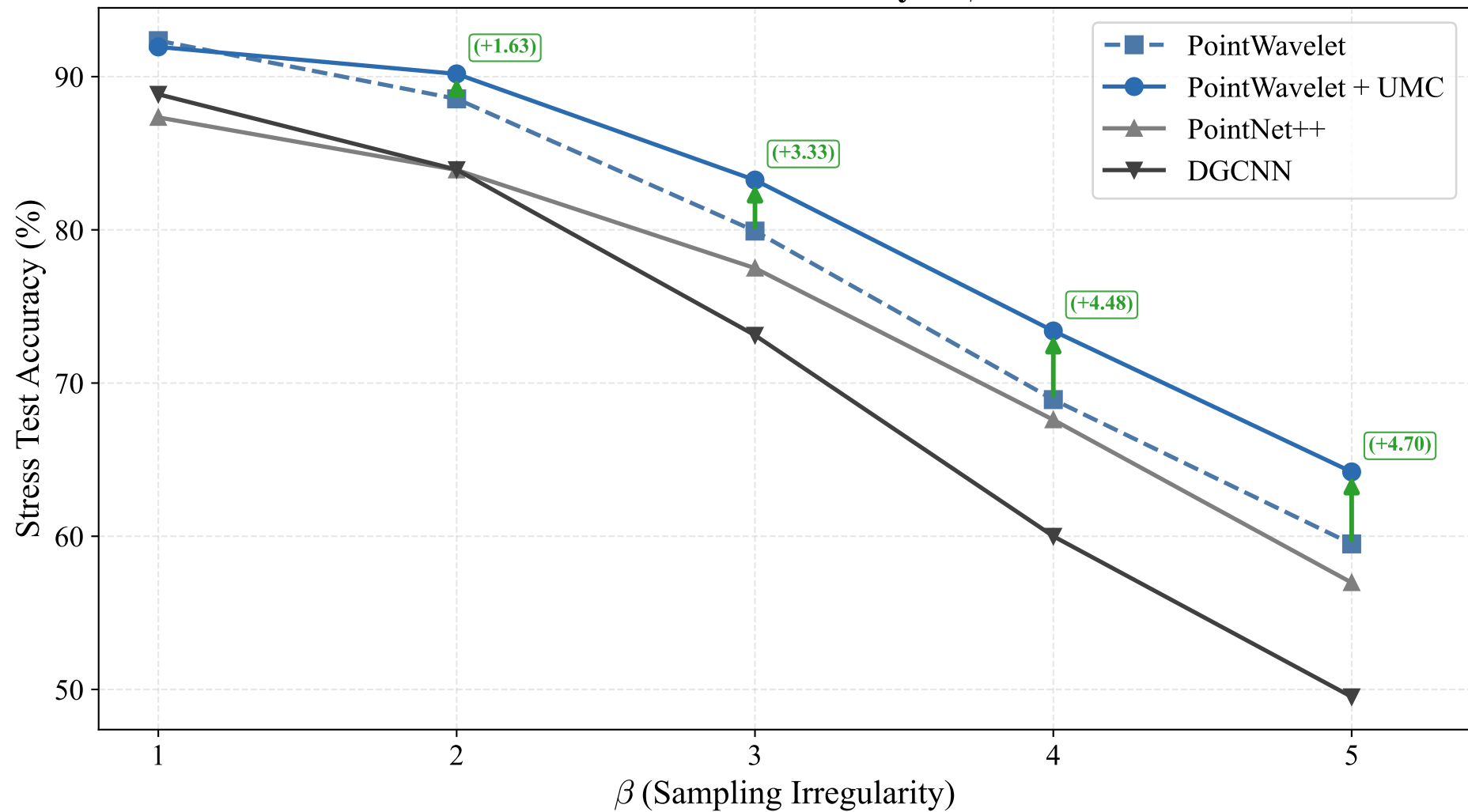
Stress Test Accuracy vs \beta
