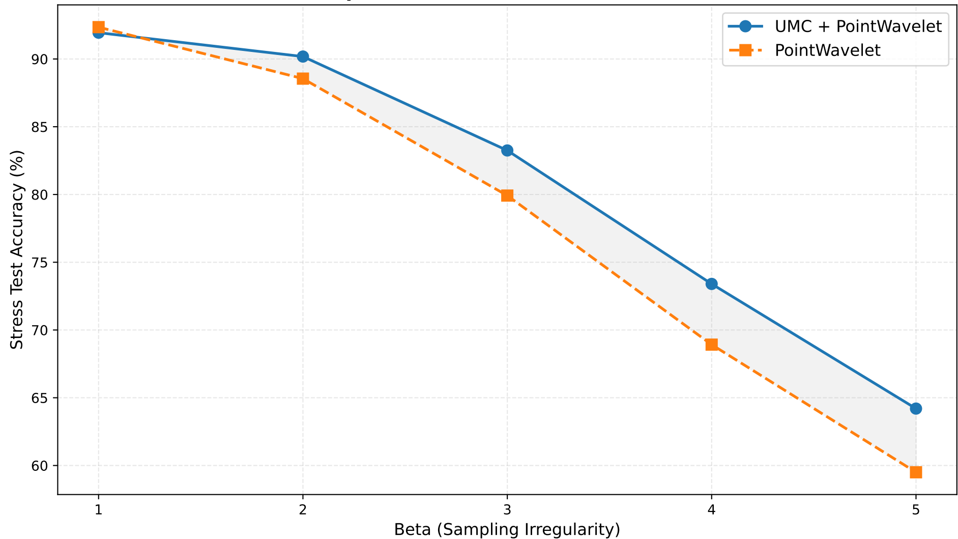
Stress Test Comparison: UMC + PointWavelet vs PointWavelet
