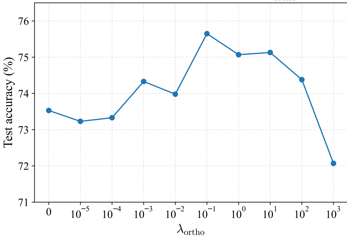
ModelNet40 Performance vs. \lambda_{\text{ortho}}
