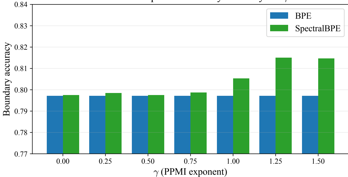
LADEC compound boundary accuracy vs. \gamma
