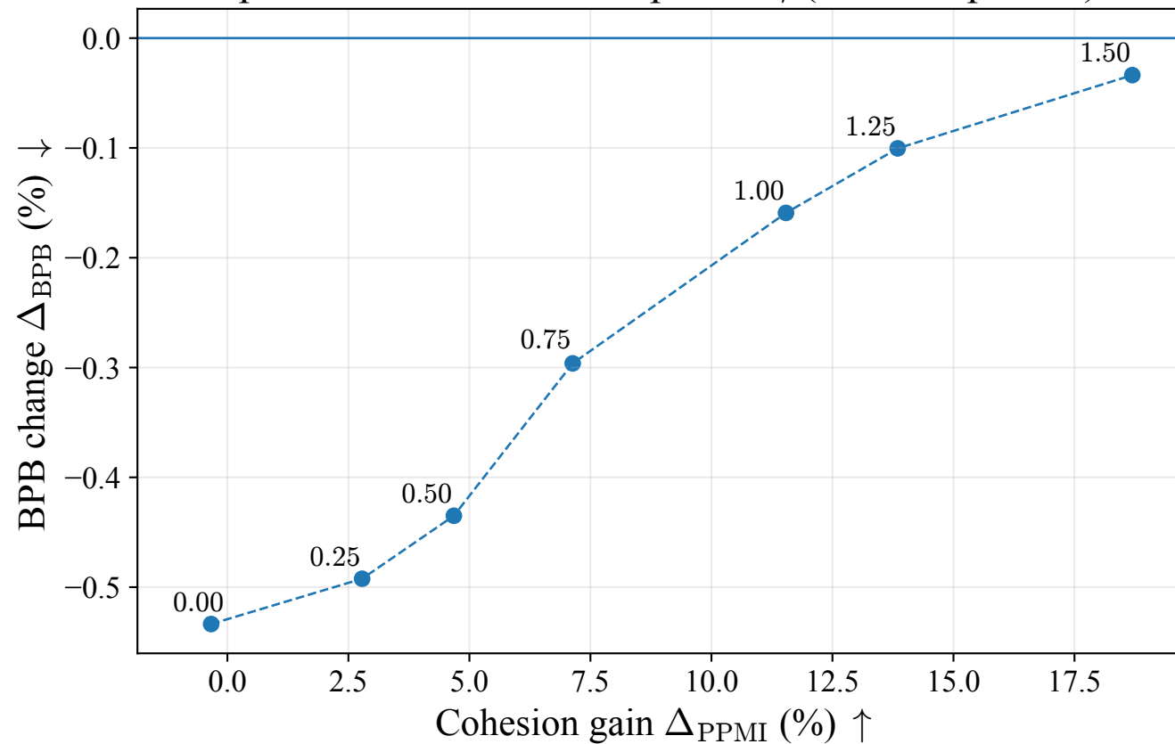
SpectralBPE Pareto sweep over \gamma (PPMI exponent)
