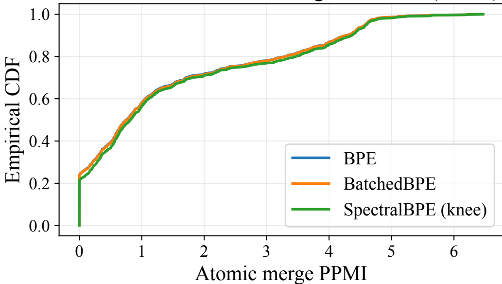
Distribution of atomic-merge cohesion (PPMI)
