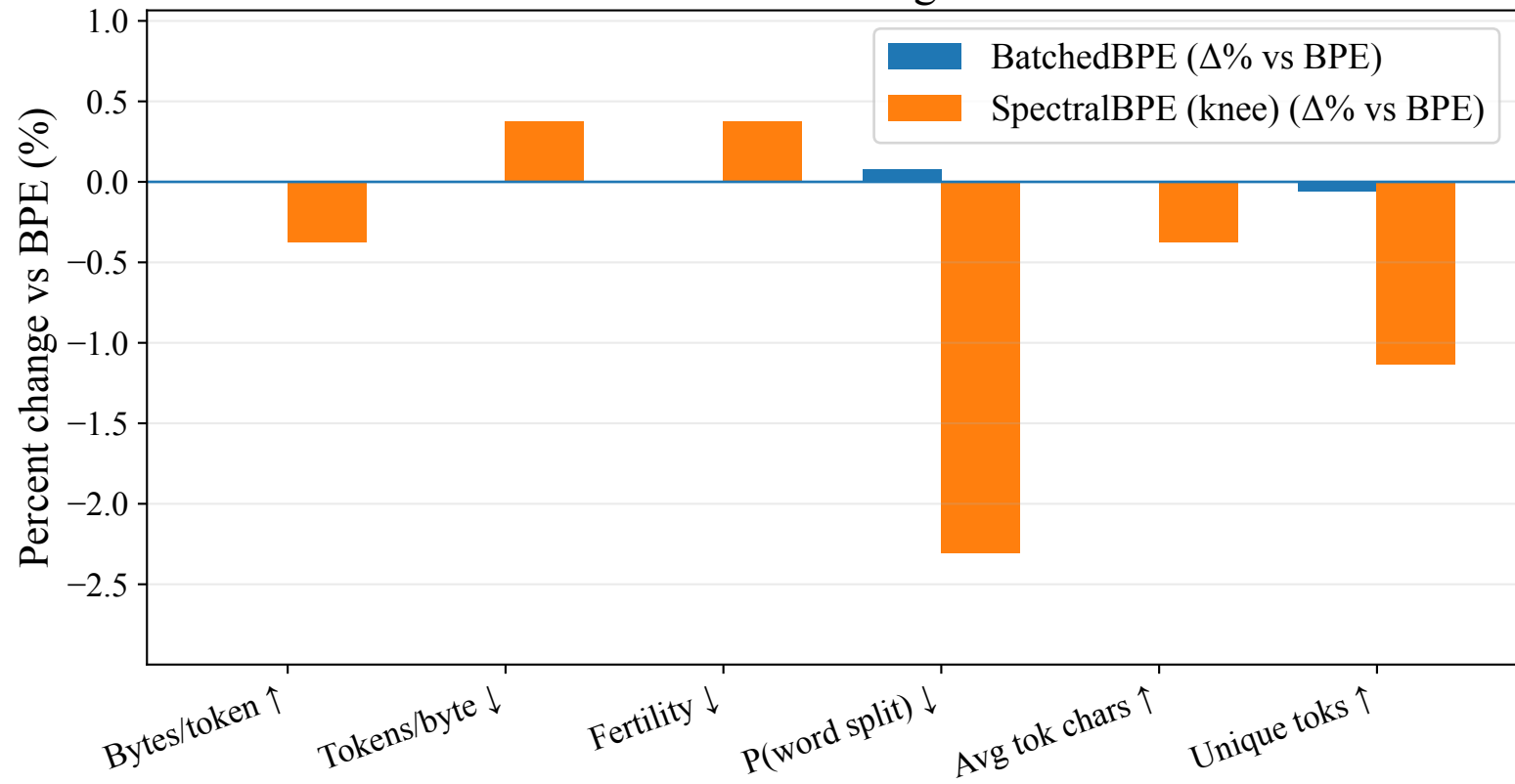
Intrinsic metric changes vs. BPE
