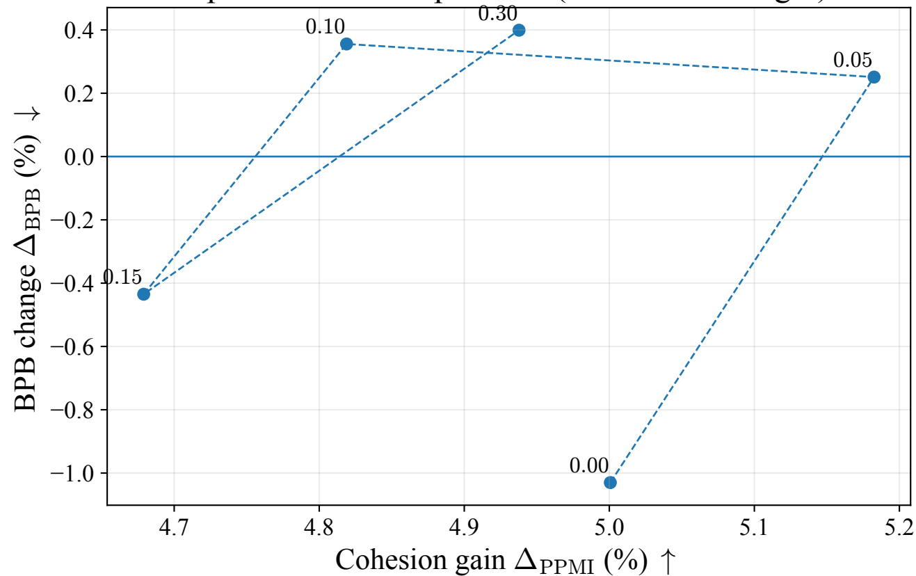
SpectralBPE sweep over \lambda (coherence strength)
