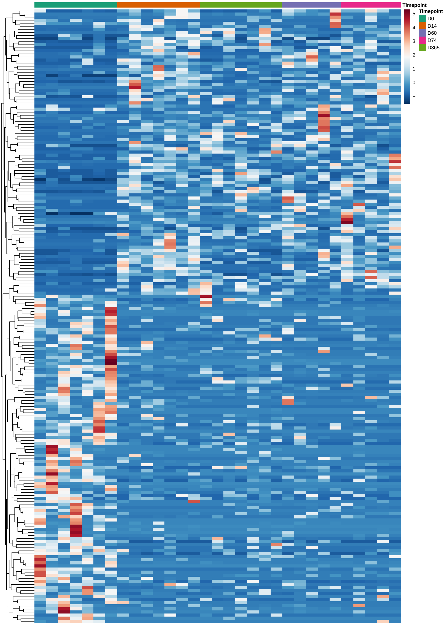
RZV CD4+ T Cell Response: Top 200 DEGs by Mean |LFC|
