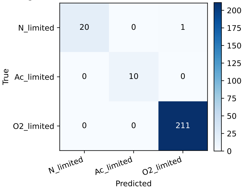
Regime classification — 5-fold CV confusion matrix
