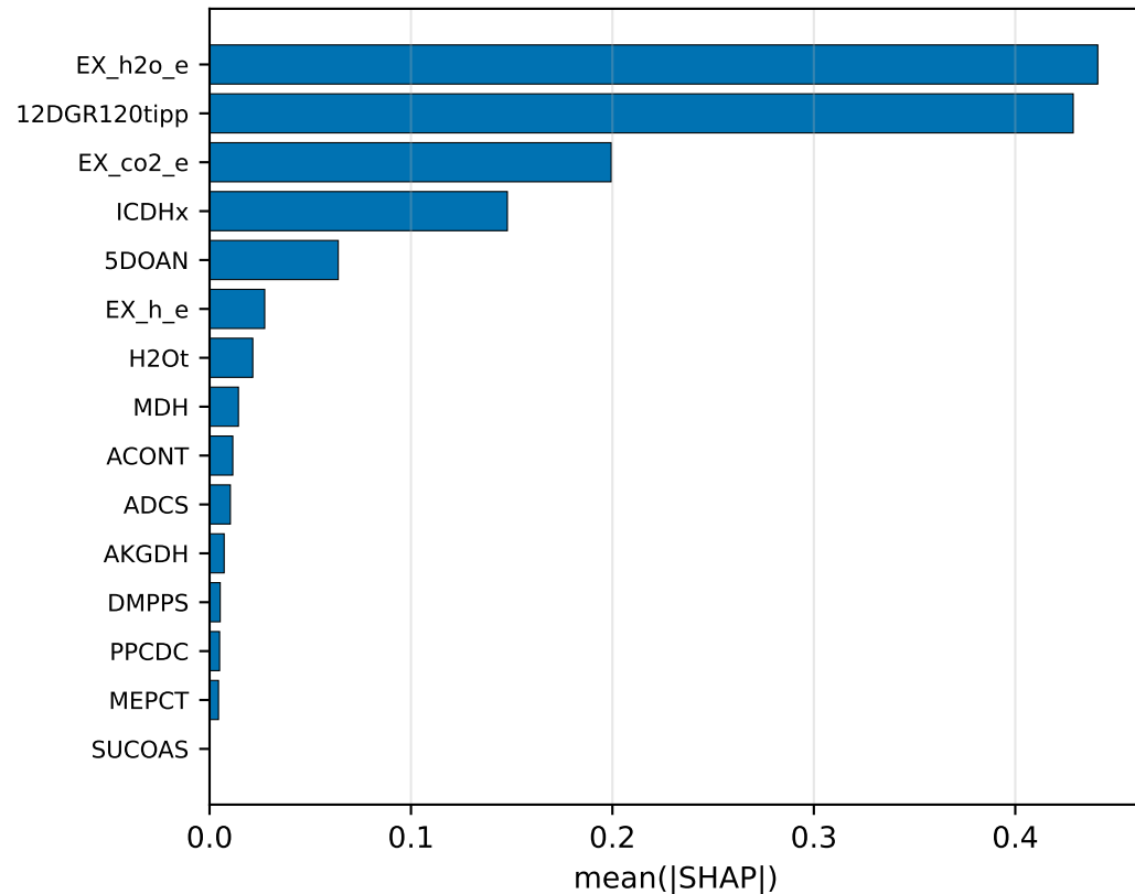
iSO1_933 (this study) — top 15 SHAP
