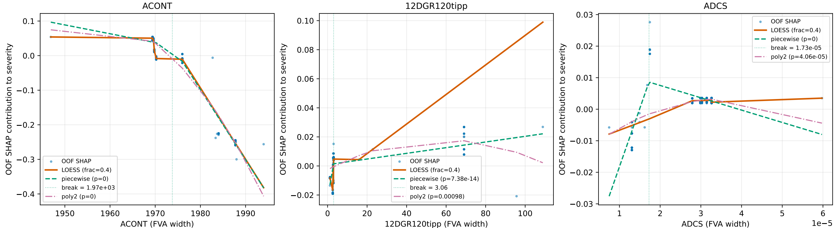
Fig 5 SHAP dependence with non-linearity diagnostics (LOESS / piecewise / poly2 vs linear; OOF 5-fold; workflow #D). Verdict = STRONG_NONLINEAR.
