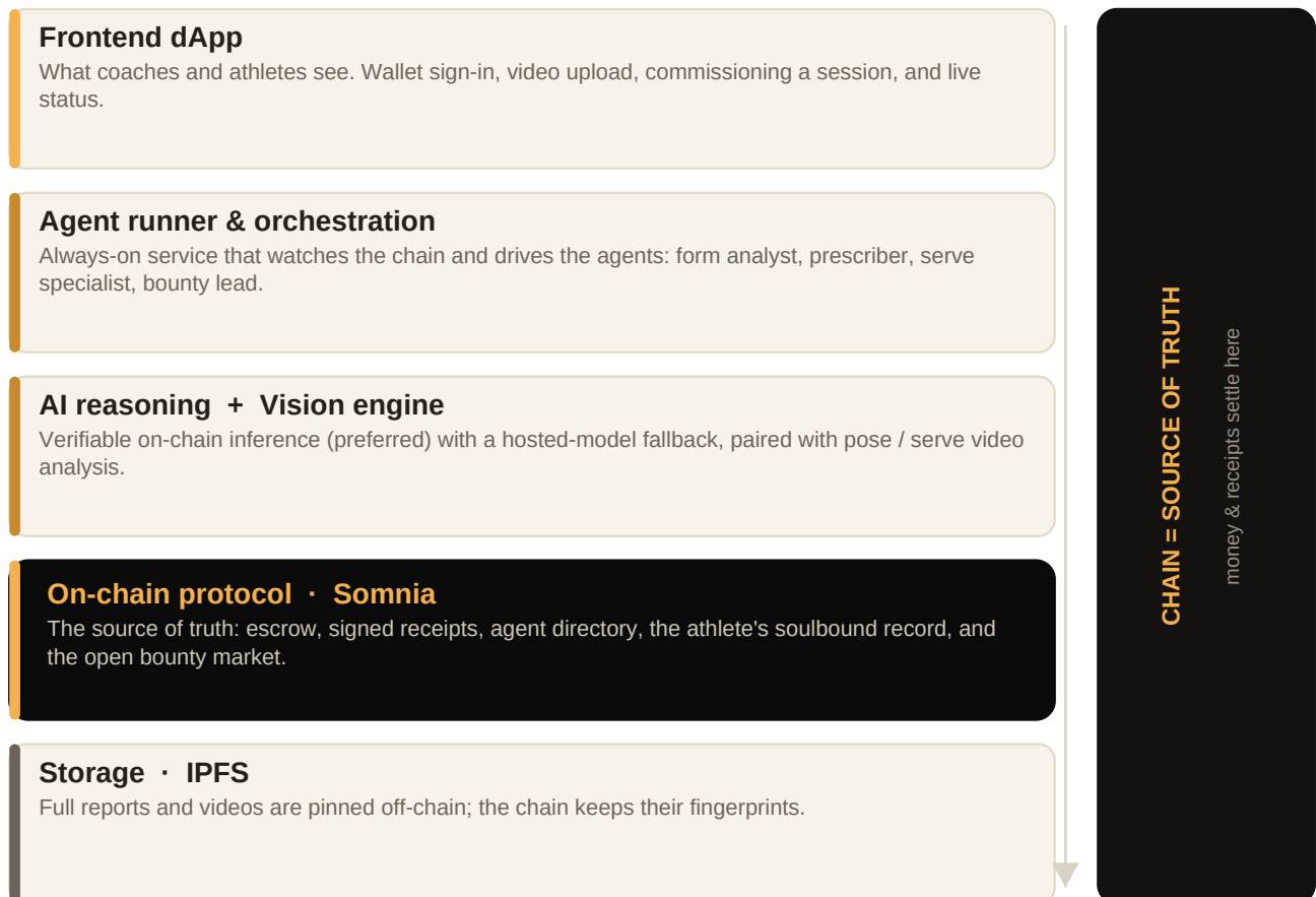
Figure 1 — The layered architecture. The frontend, agent runner, AI and vision services all do work off-chain, then write signed results back to the chain, which holds escrow and the canonical record.
