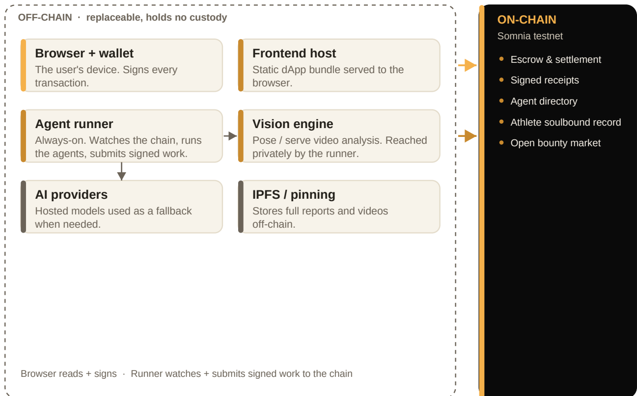
Figure 5 — Deployment topology and trust boundary. The browser reads the chain and signs transactions through the user's wallet; the always-on runner watches the chain, calls the off-chain services, and submits signed work back on-chain.
