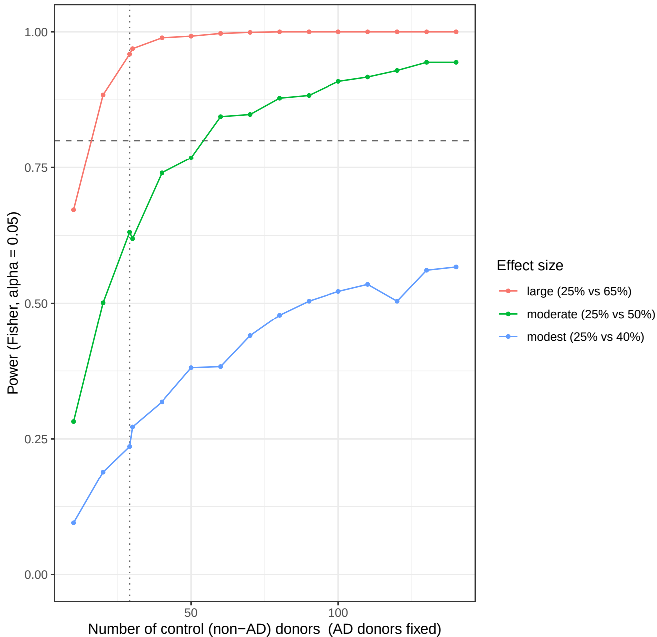
Power to detect an AD prevalence difference vs # controls
