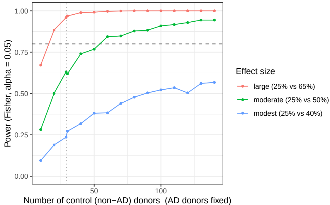
Power to detect an AD prevalence difference vs # controls
