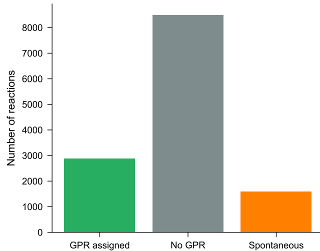
d Gene-Reaction Coverage
