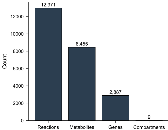
a Human-GEM Model Statistics
