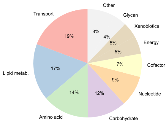
c Reactions by Subsystem
