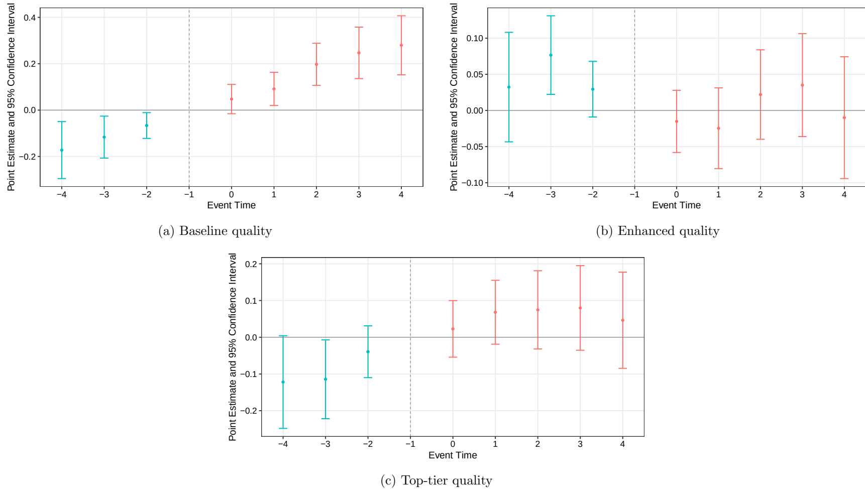
Figure A.12: Event study estimates: first-year enrollment by institutional quality.
