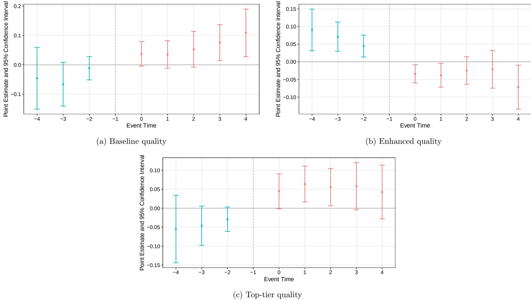
Figure A.6: Event study estimates: declared slots by institutional quality.
