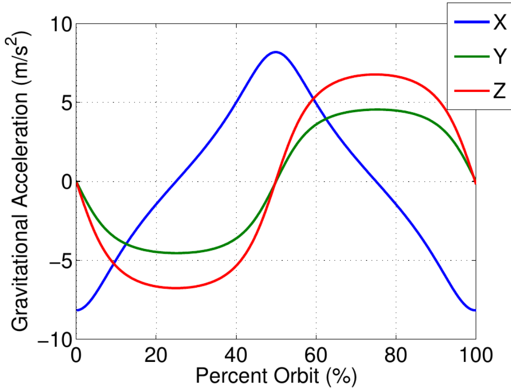
Figure 7.4.1 Gravitational Field of Earth in Inertial Frame for 56 Degree Orbit at 600 km Above Surface
