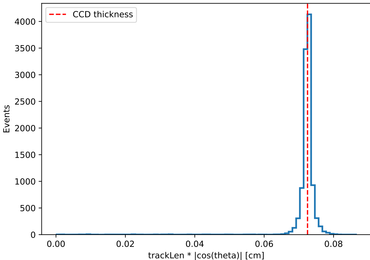
L \cdot \cos(\theta) vs CCD thickness
