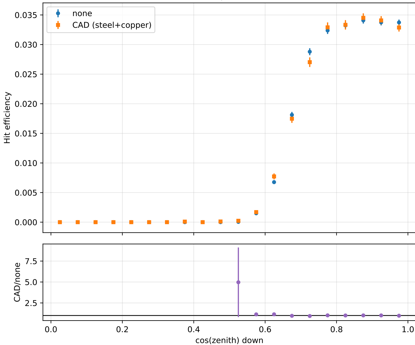
Hit efficiency vs \cos(\text{zenith})
