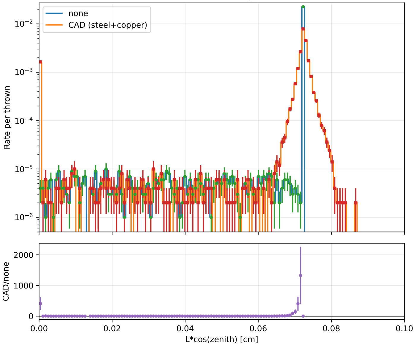
Lcos distribution (hits, per thrown)
