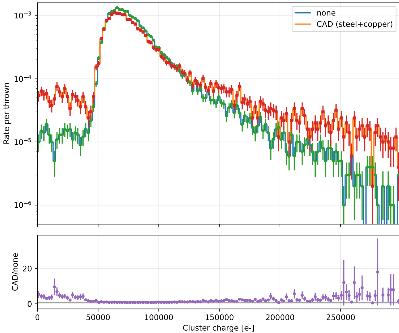
Charge distribution (hits, core)
