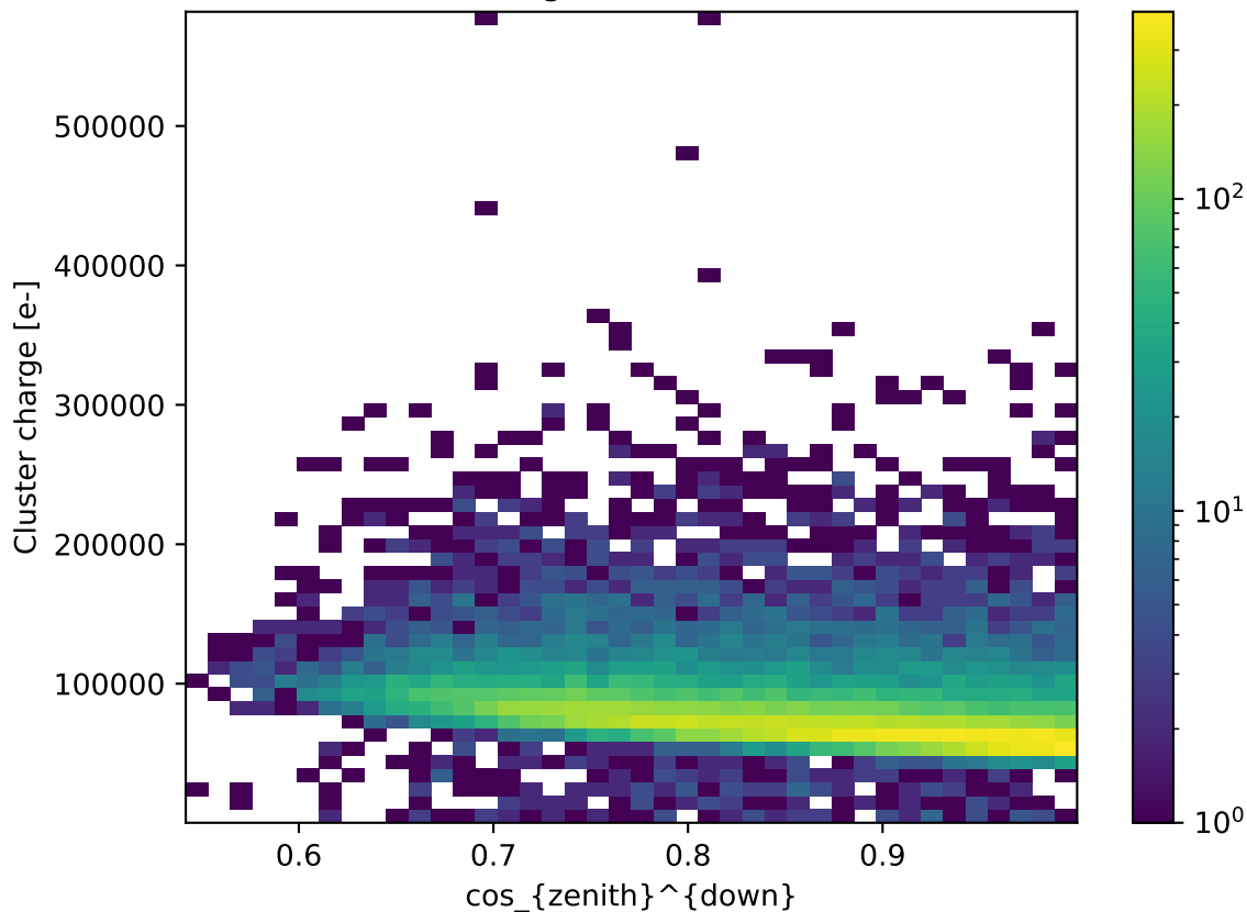
Cluster charge vs \cos(\text{zenith}) (tail)
