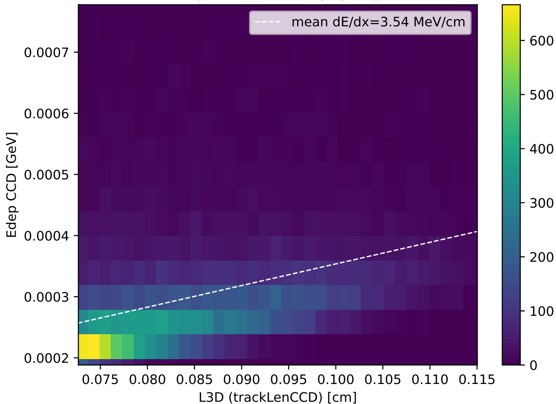
Edep vs L3D (throughgoing)
