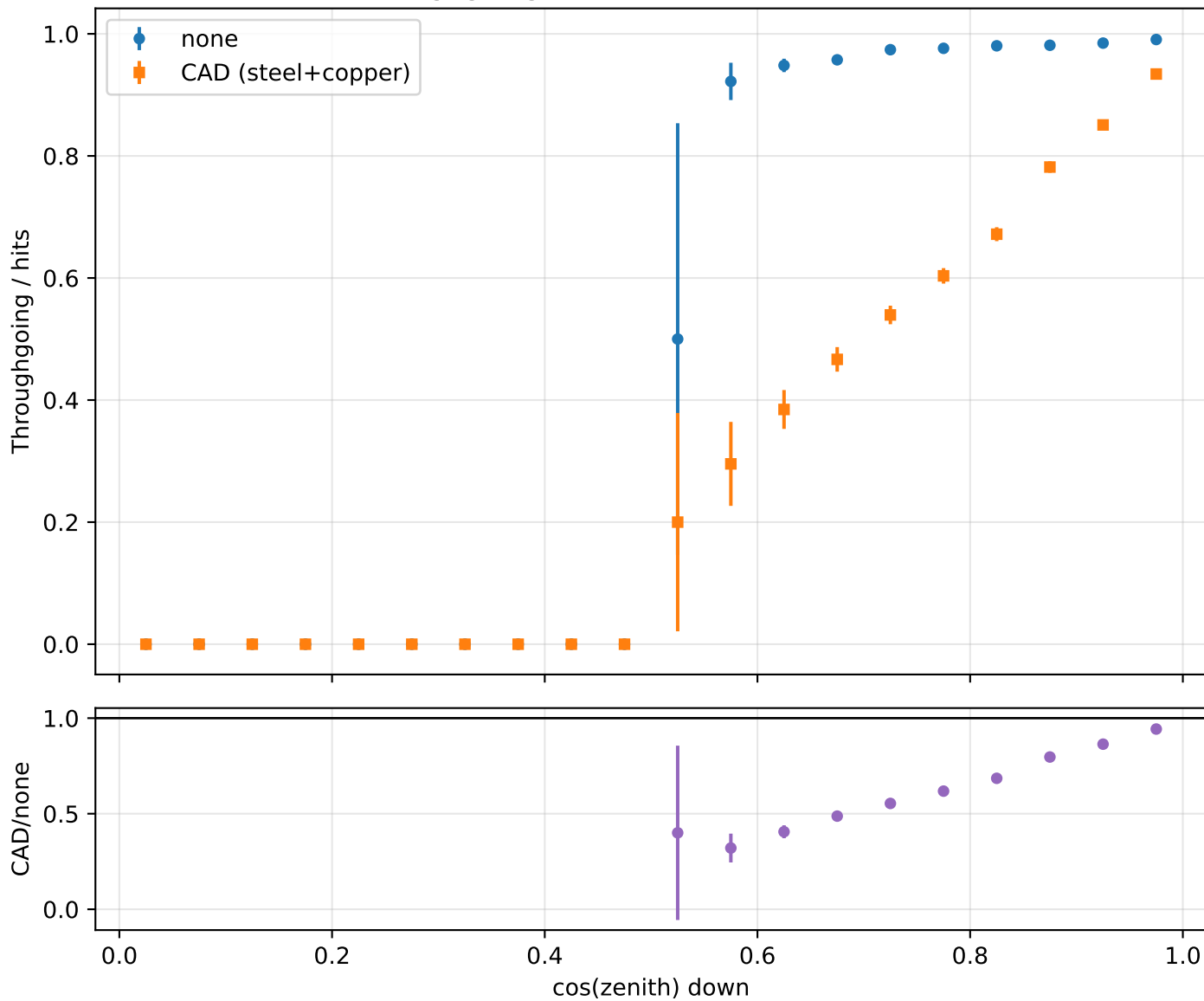
Throughgoing fraction of hits vs \cos(\text{zenith})
