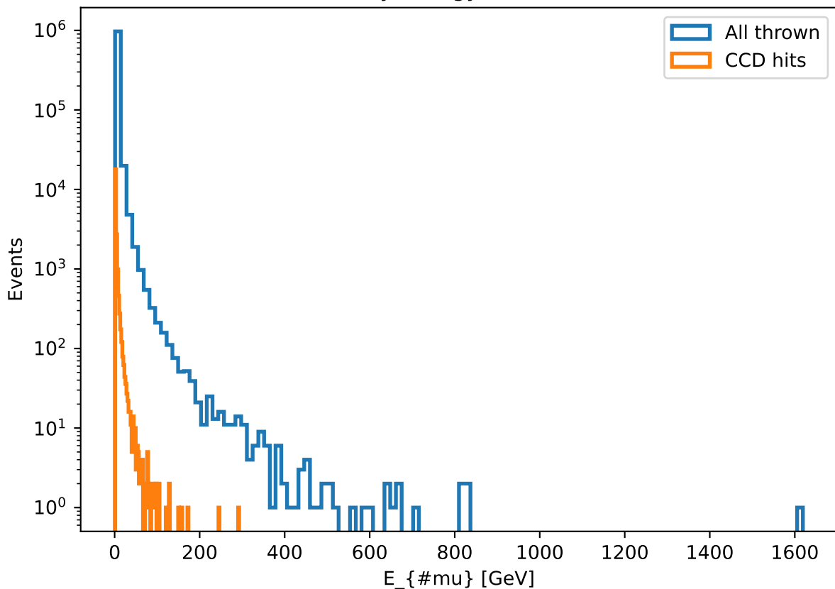
Primary energy (all vs hits)
