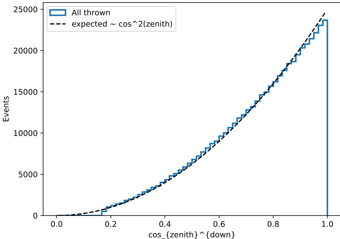
Downward cos(zenith) all thrown (clamp low=0, high=0)
