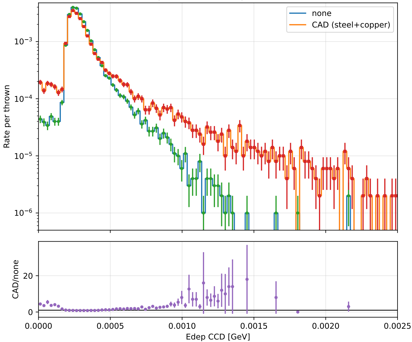
Edep CCD core (hits, per thrown)
