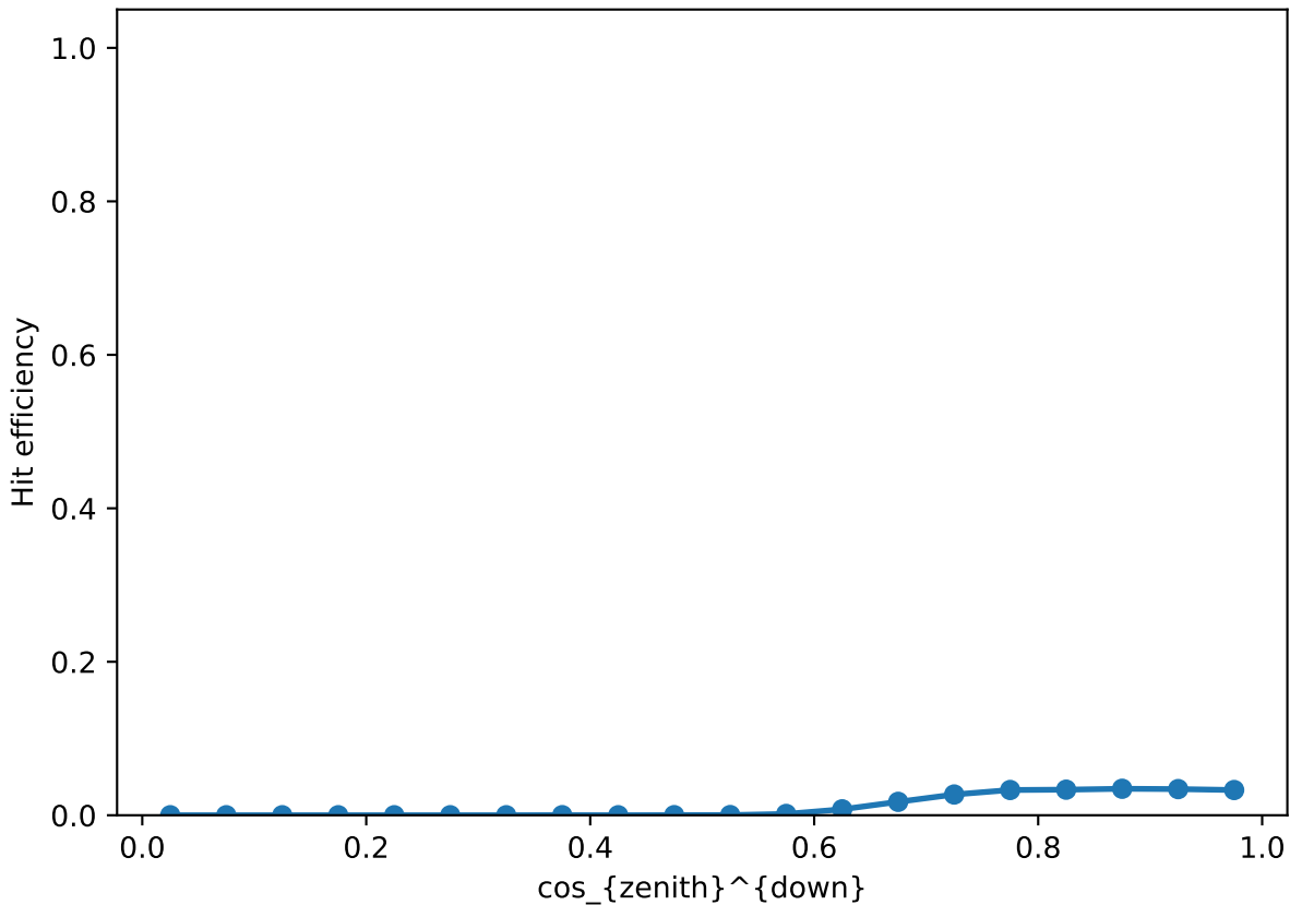
CCD hit efficiency vs \cos(\text{zenith})
