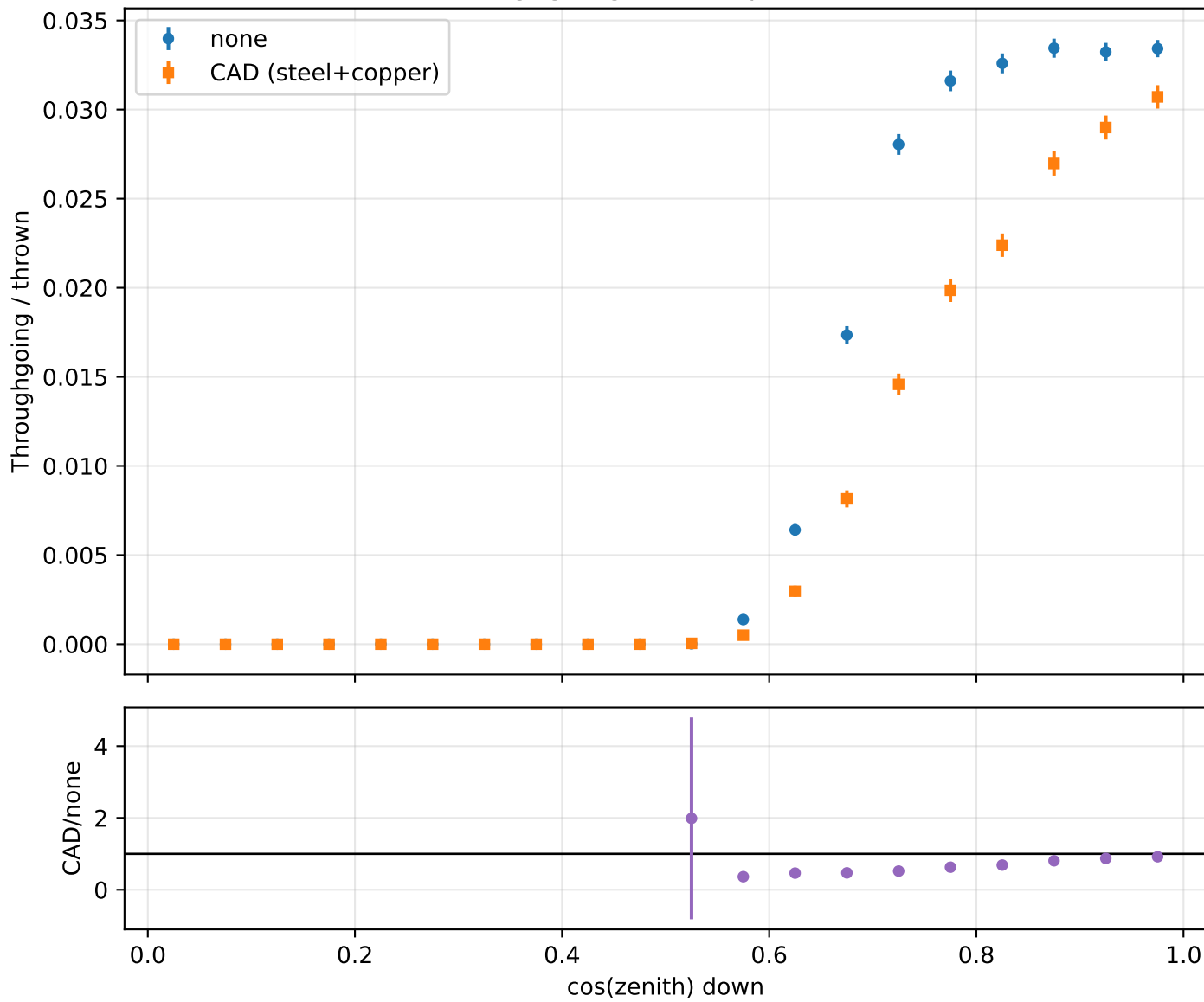
Throughgoing fraction per thrown
