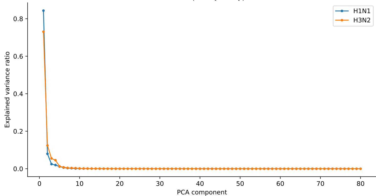
PCA scree plot by subtype
