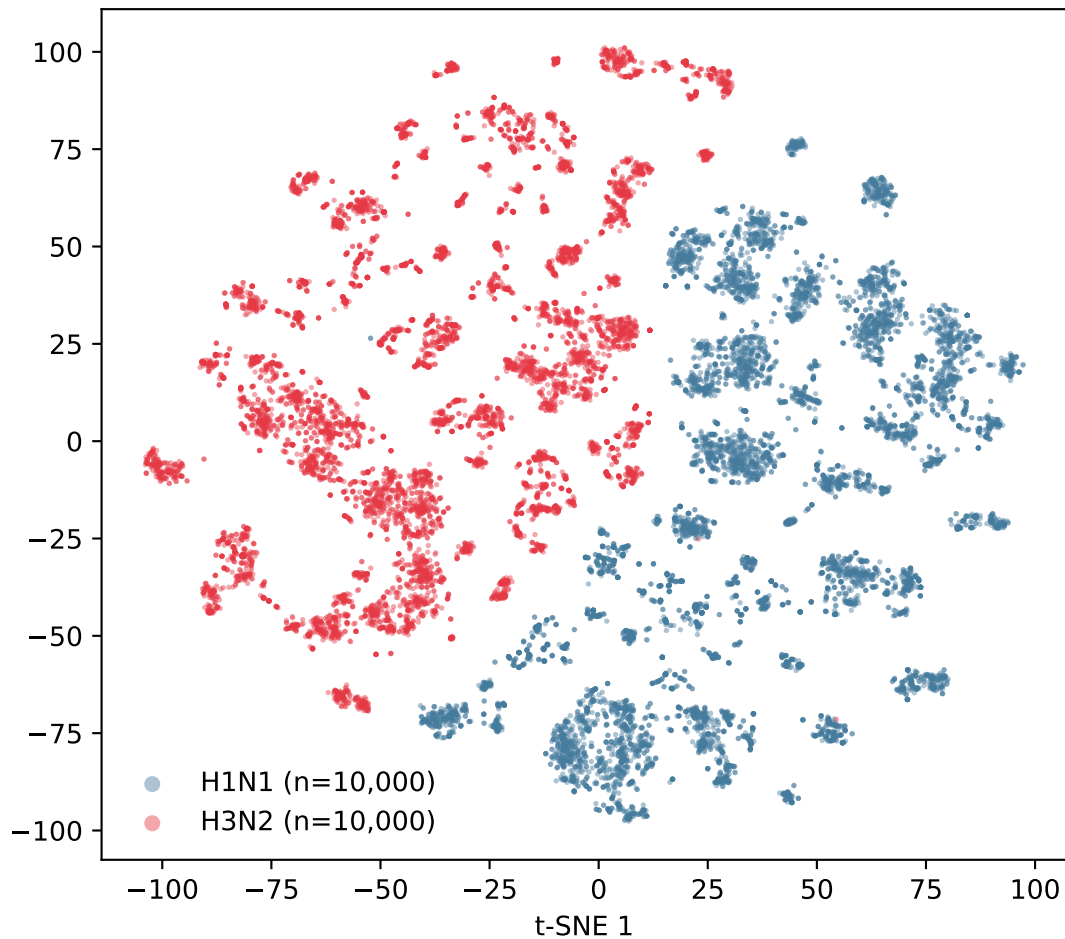
t-SNE by subtype
