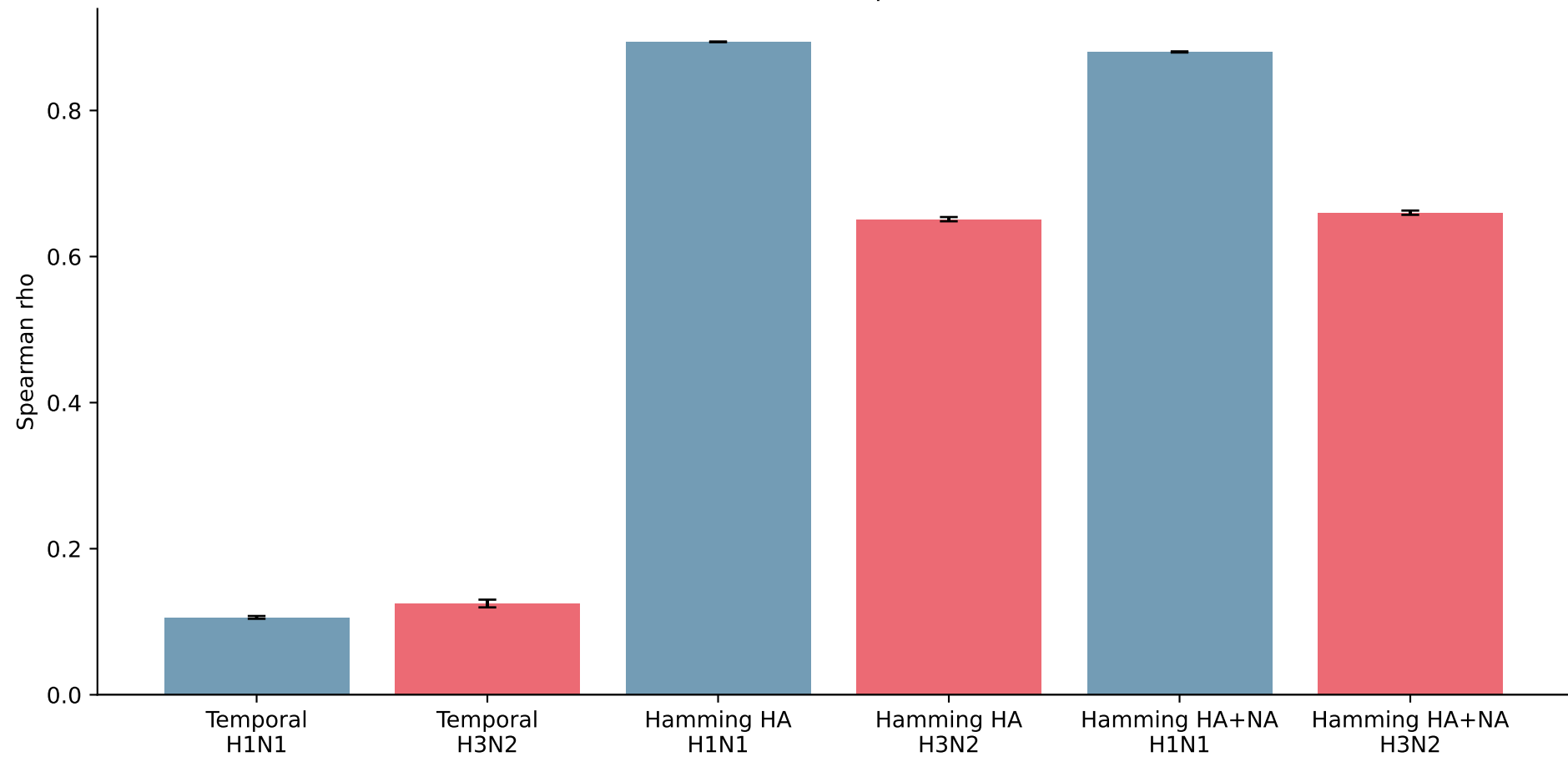
Latent distance correlation with temporal and molecular distances
