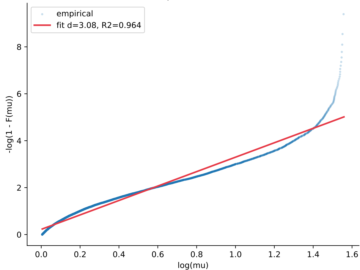
TwoNN fit example (n=20,000, trim=0.05)
