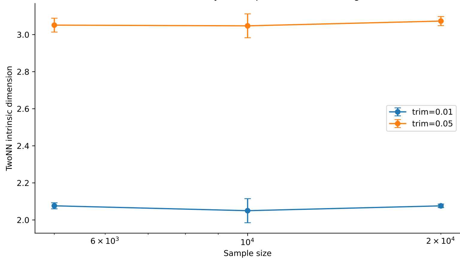
TwoNN sensitivity to sample size and trimming
