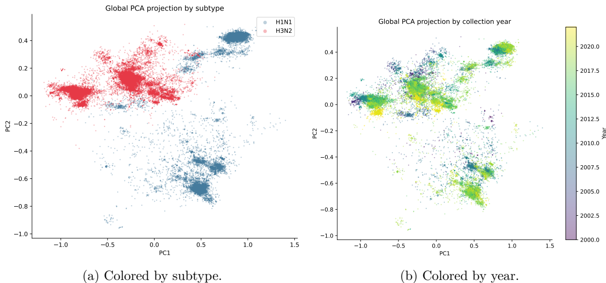
Figure 6: Two-dimensional global PCA projection. The projection is descriptive and should not be read as a complete representation of evolutionary or antigenic relationships. In particular, this two-dimensional view does not constitute quantitative phylogenetic, antigenic, or forecasting evidence.
