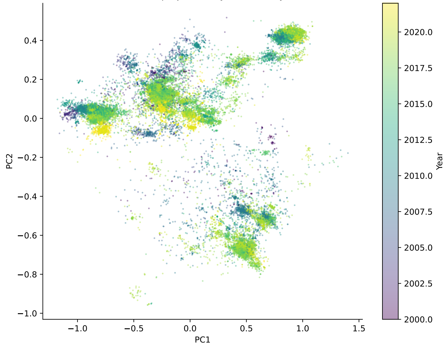
Global PCA projection by collection year
