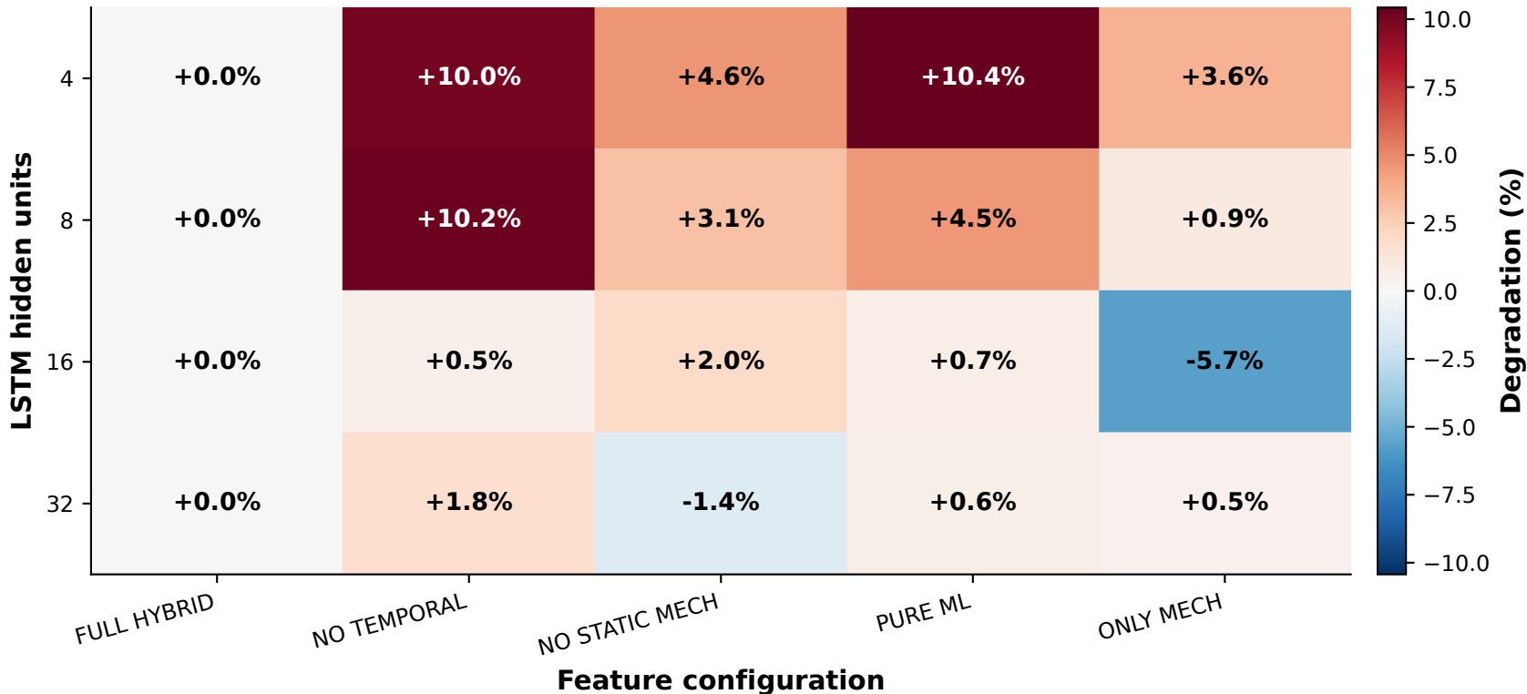
LSTM capacity heatmap: mean MAE degradation (%) from Full Hybrid (n=10 seeds per cell)
