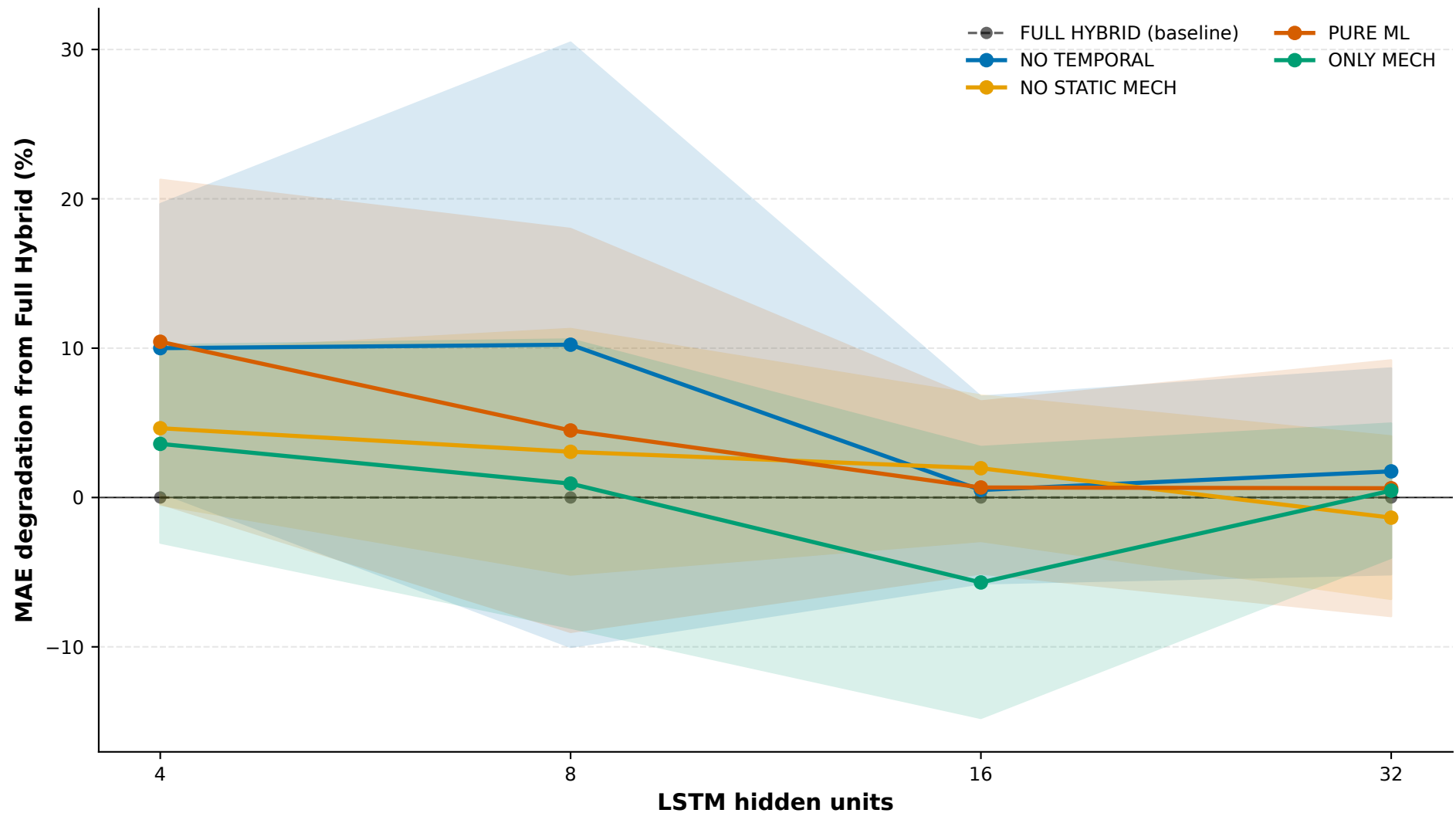
LSTM capacity sweep: feature contribution vs model size (n=10 seeds per cell)
