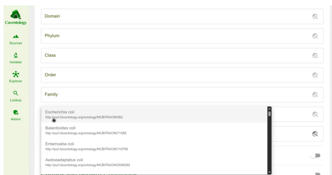
Fig. 12. Caventology Add Isolate Page - Ontology Suggestions
