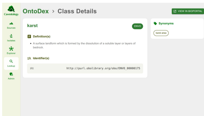
Fig. 14. Caventology OLS Details Page
