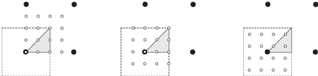
Figure 5: Integration grids for a 2D square lattice ( density). Left/Center: Unshifted grid with 6 inequivalent IBZ points (gray). Right: Shifted special-point grid with only 3 inequivalent points.
