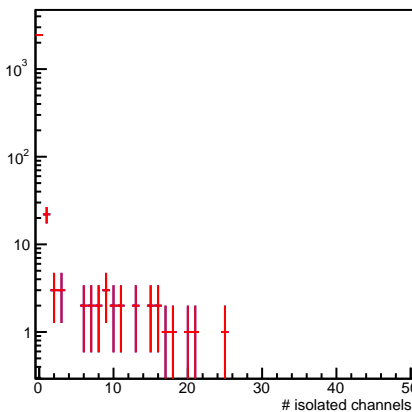
# isolated channels
