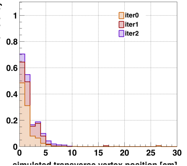
CMS Simulation, 2016, \sqrt{s}=13 TeV, Private
