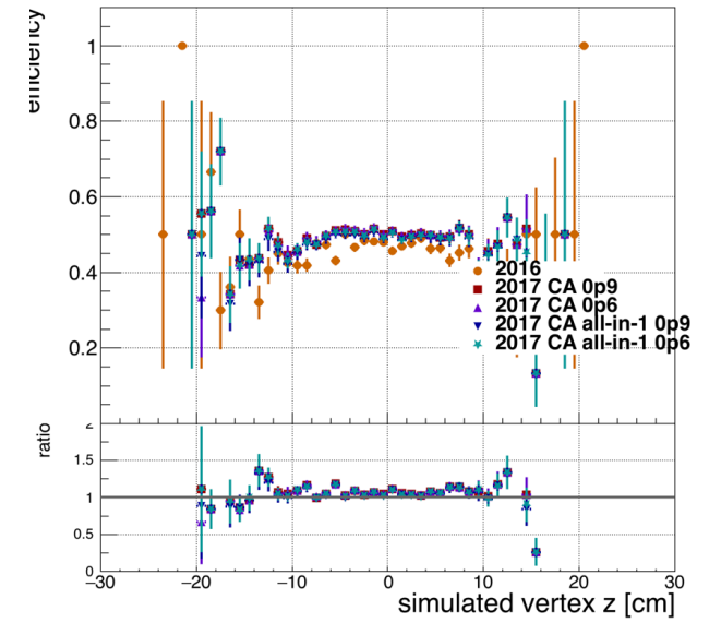
CMS Simulation, 2016, \sqrt{s}=13 TeV, Private
