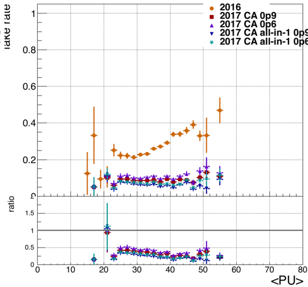
CMS Simulation, 2016, \sqrt{s}=13 TeV, Private
