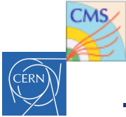
CMS Simulation, 2016, \sqrt{s}=13 TeV, Private
