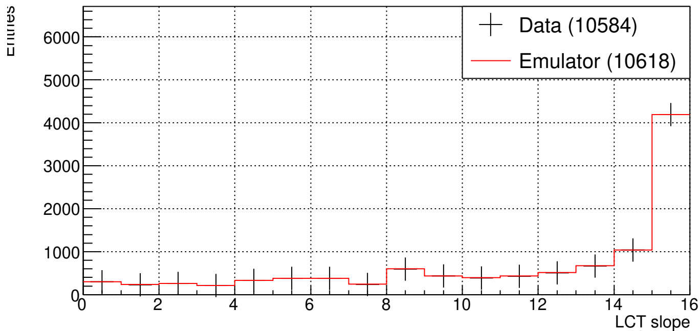
ME21 LCT slope (B904 Cosmic Run 211105_132717)
