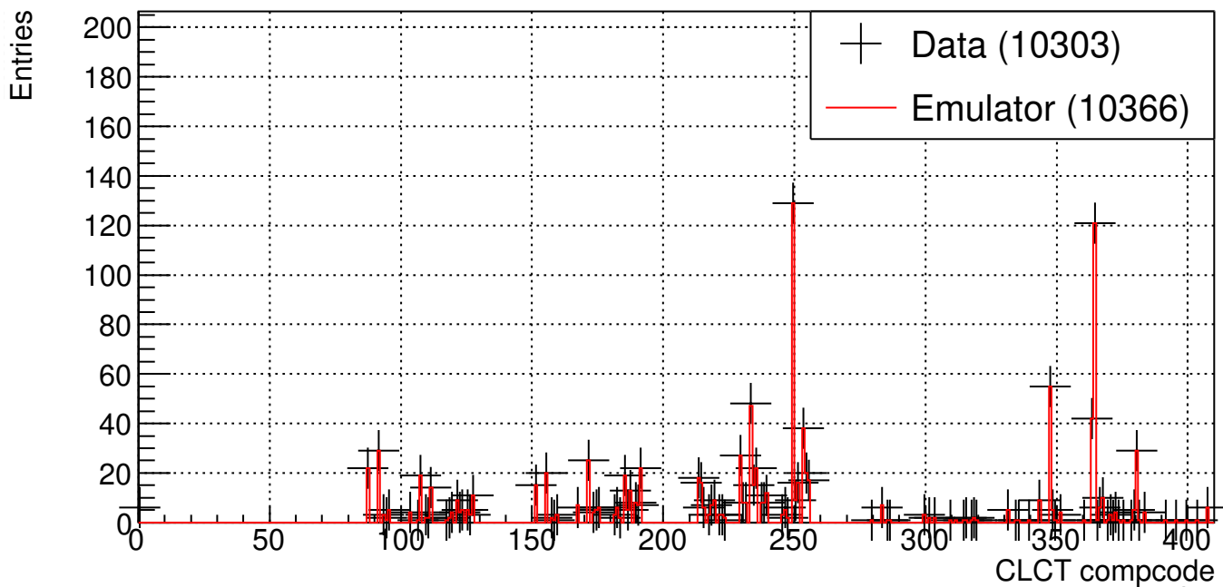
ME21 CLCT compcode (B904 Cosmic Run 211105_132717)
