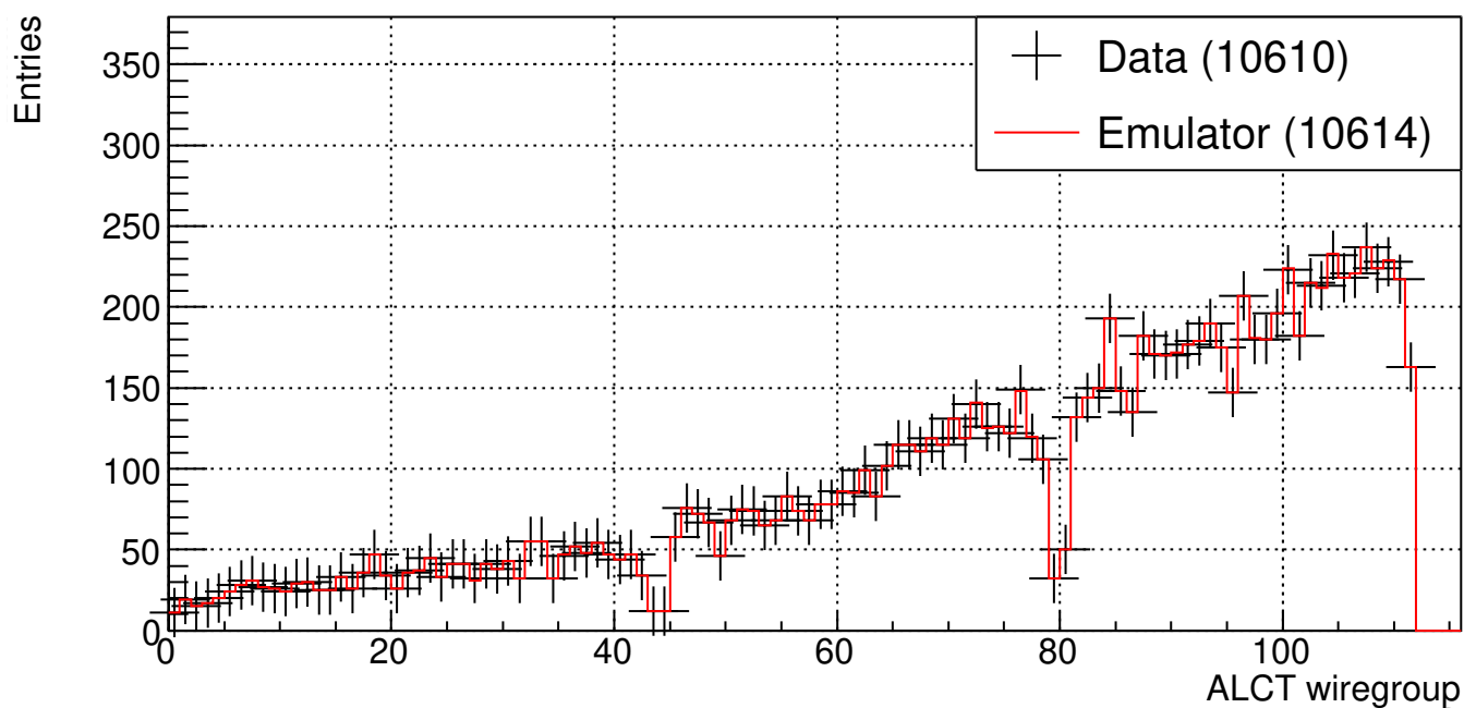
ME21 ALCT wiregroup (B904 Cosmic Run 211105_132717)
