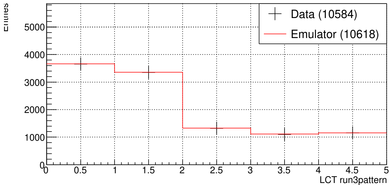
ME21 LCT run3pattern (B904 Cosmic Run 211105_132717)
