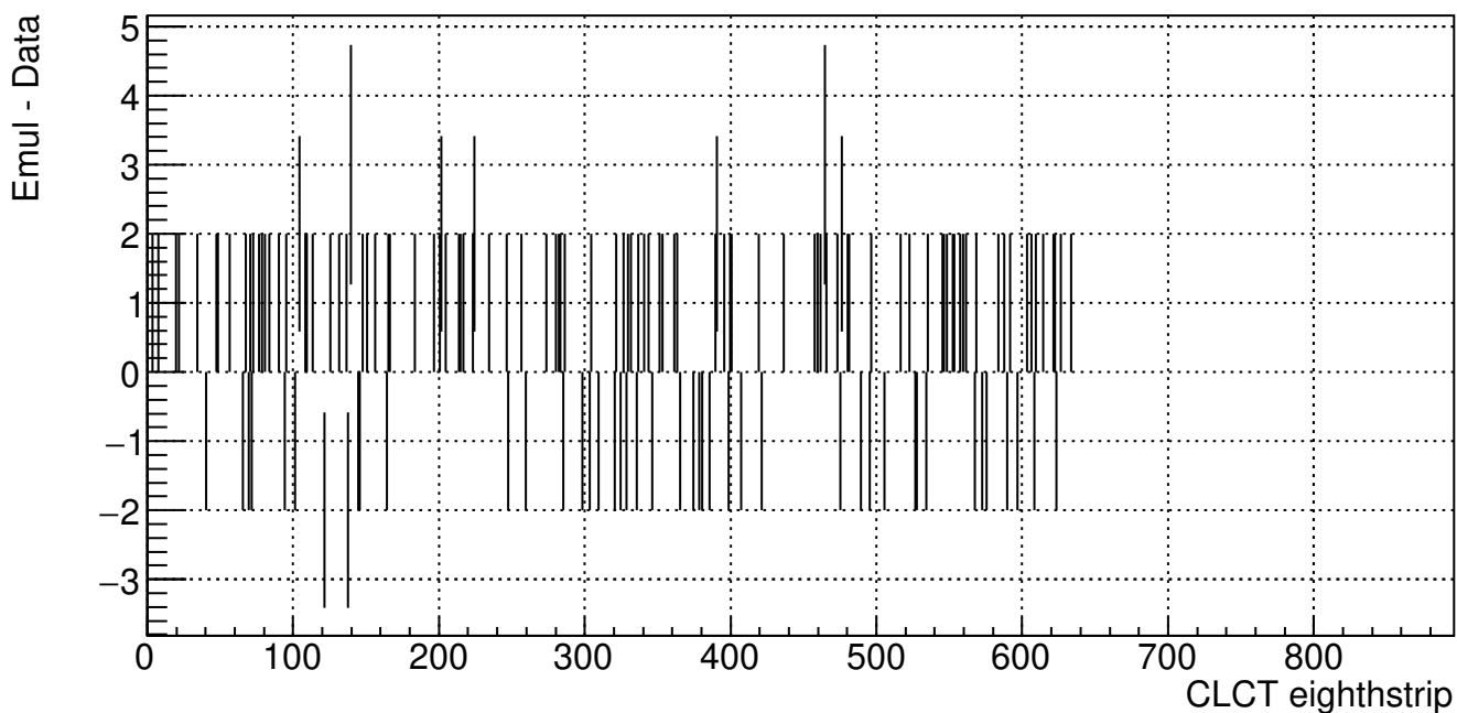
ME21 CLCT eighthstrip (B904 Cosmic Run 211105_132717)
