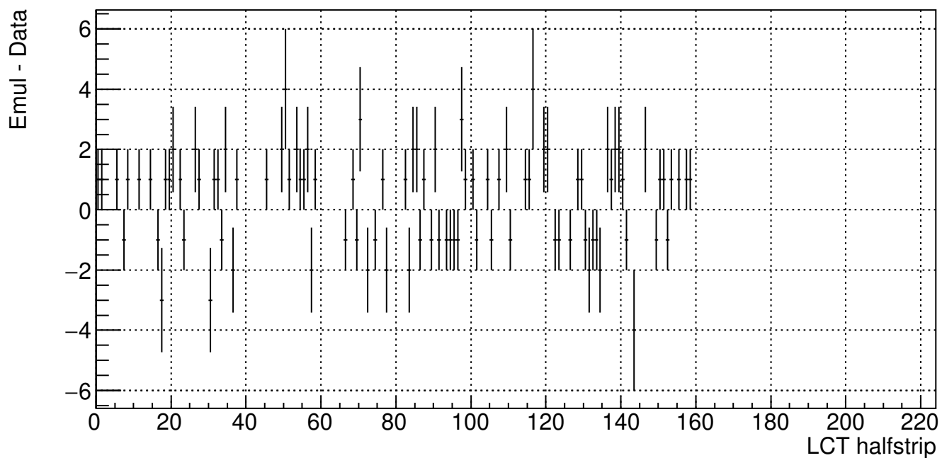
ME21 LCT halfstrip (B904 Cosmic Run 211105_132717)
