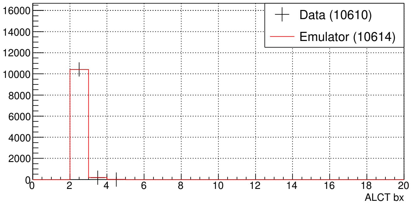
ME21 ALCT bx (B904 Cosmic Run 211105_132717)
