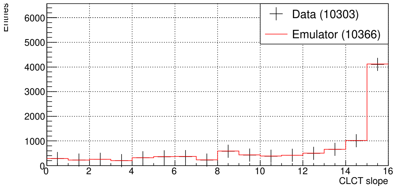
ME21 CLCT slope (B904 Cosmic Run 211105_132717)
