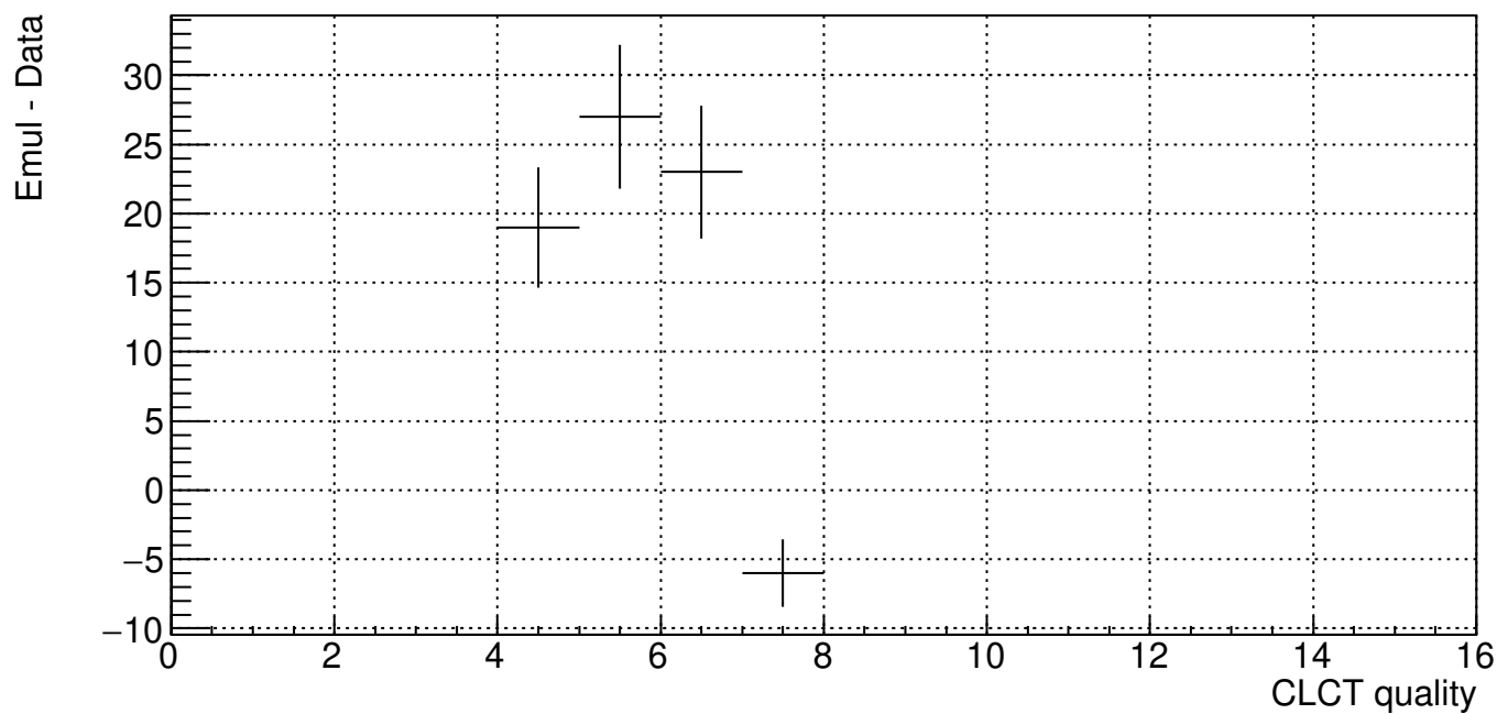
ME21 CLCT quality (B904 Cosmic Run 211105_132717)
