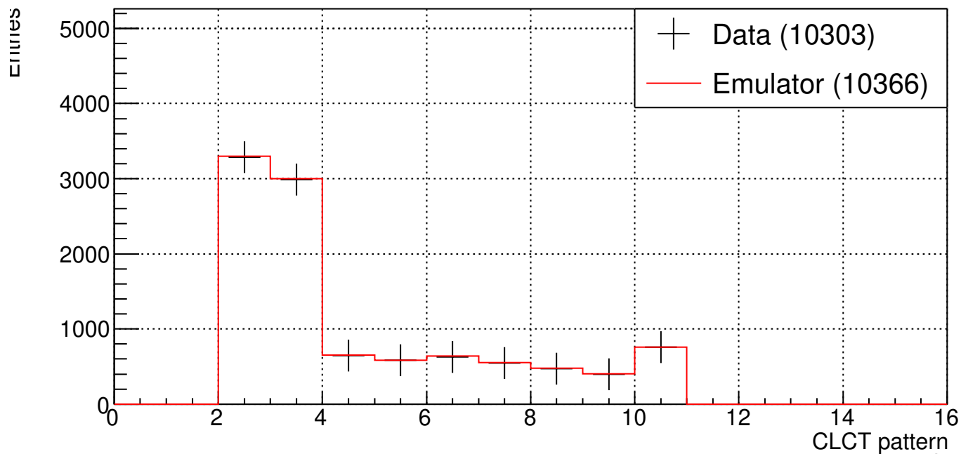
ME21 CLCT pattern (B904 Cosmic Run 211105_132717)
