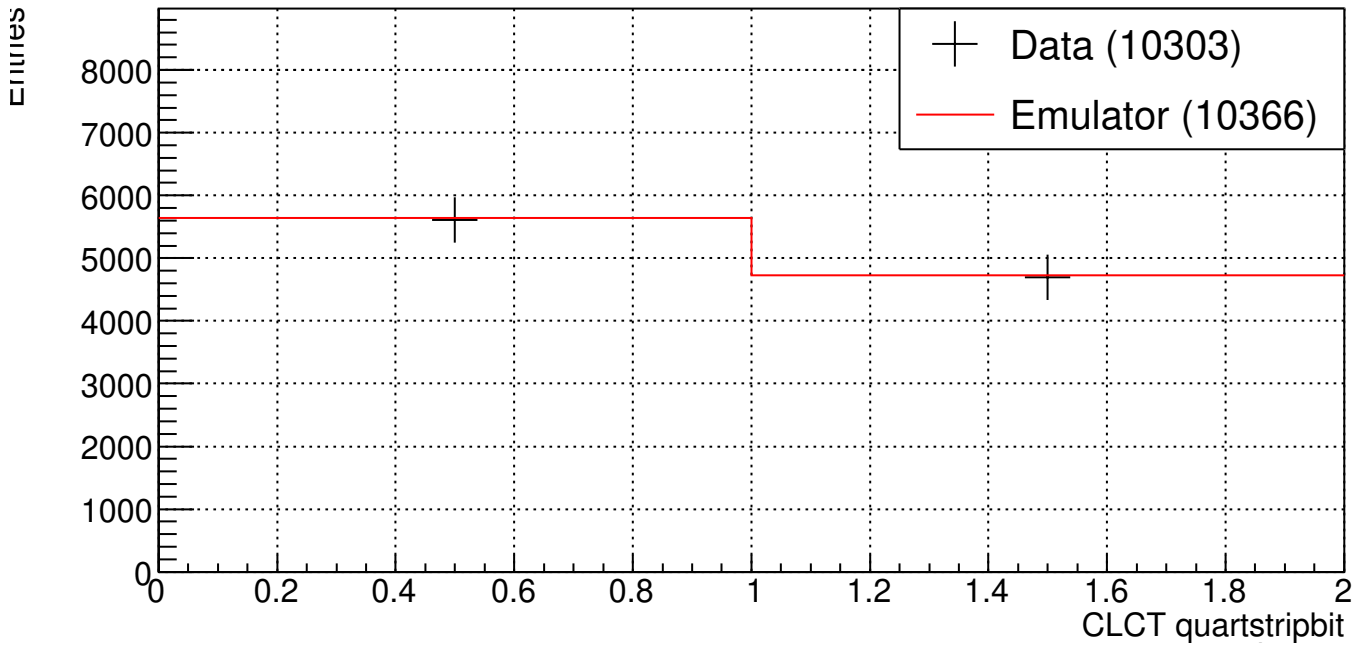
ME21 CLCT quartstripbit (B904 Cosmic Run 211105_132717)
