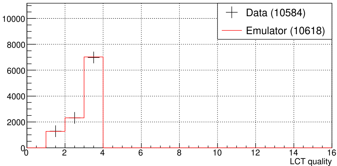
ME21 LCT quality (B904 Cosmic Run 211105_132717)
