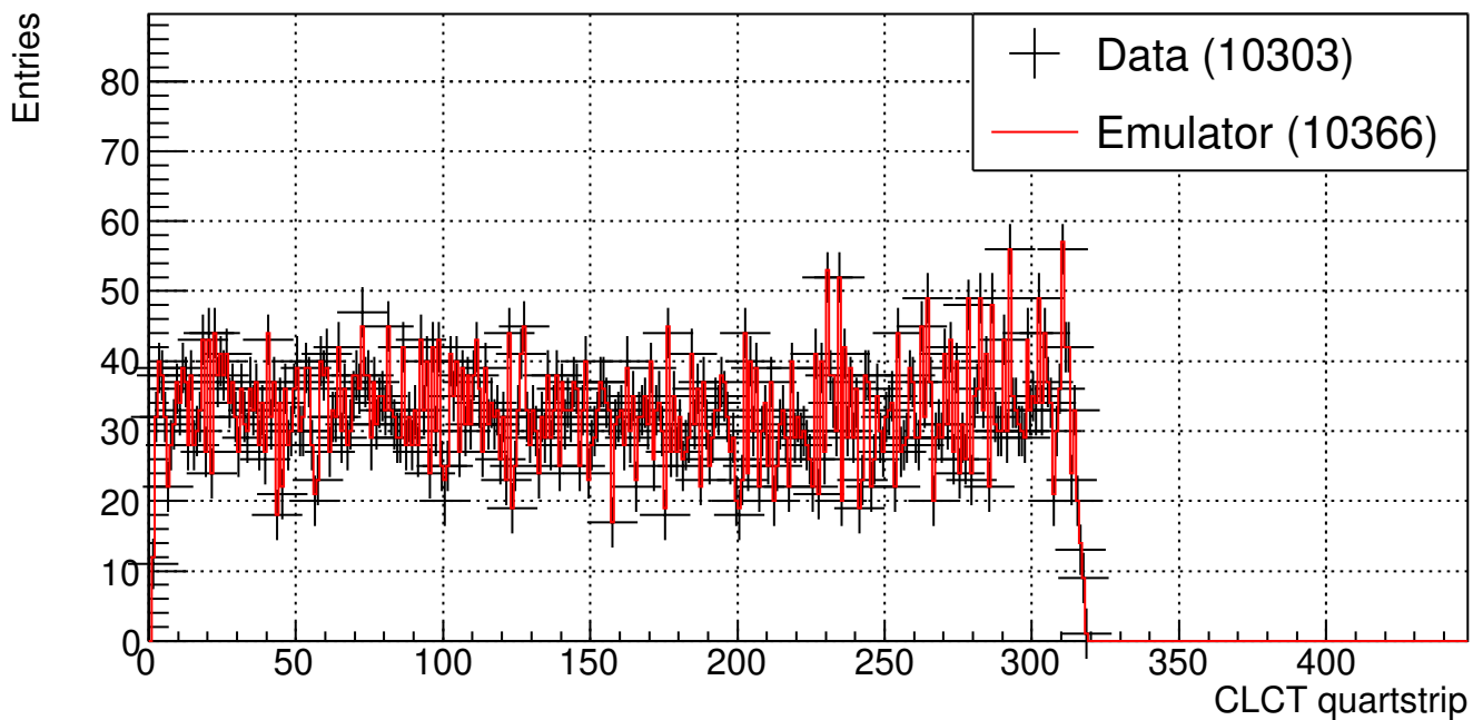
ME21 CLCT quartstrip (B904 Cosmic Run 211105_132717)
