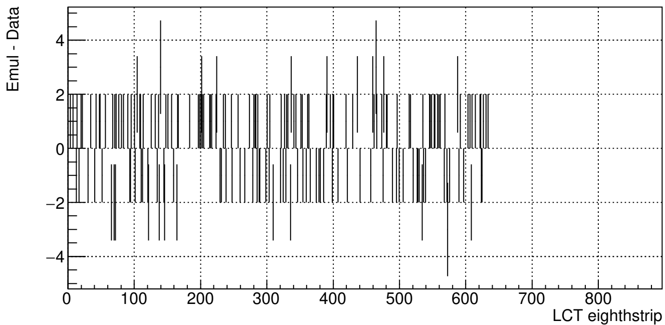
ME21 LCT eighthstrip (B904 Cosmic Run 211105_132717)
