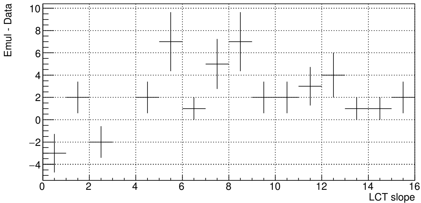
ME21 LCT slope (B904 Cosmic Run 211105_132717)
