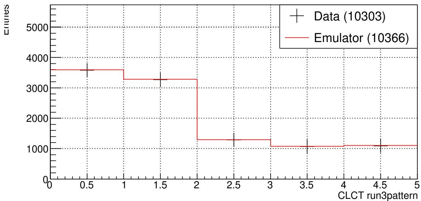
ME21 CLCT run3pattern (B904 Cosmic Run 211105_132717)
