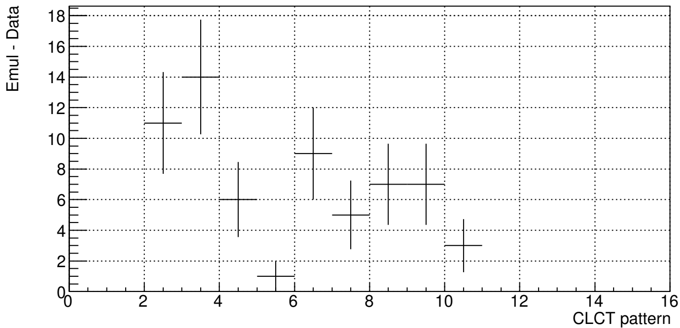
ME21 CLCT pattern (B904 Cosmic Run 211105_132717)
