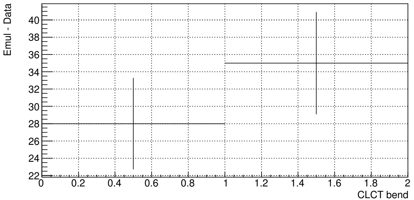
ME21 CLCT bend (B904 Cosmic Run 211105_132717)
