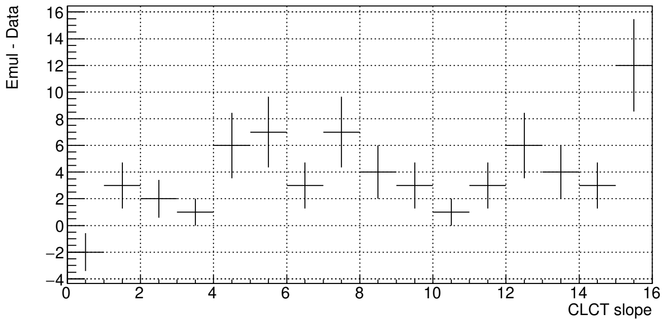
ME21 CLCT slope (B904 Cosmic Run 211105_132717)
