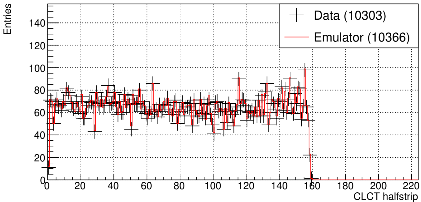
ME21 CLCT halfstrip (B904 Cosmic Run 211105_132717)
