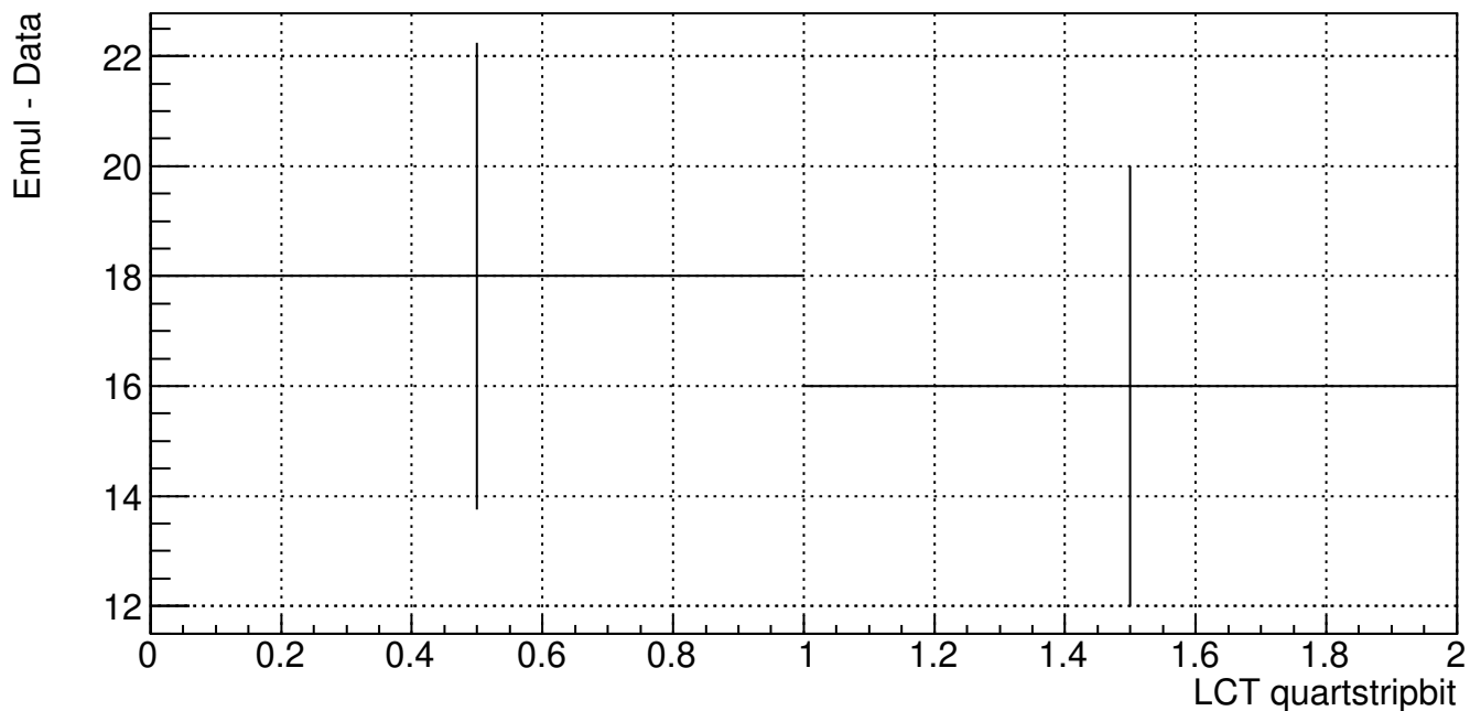
ME21 LCT quartstripbit (B904 Cosmic Run 211105_132717)
