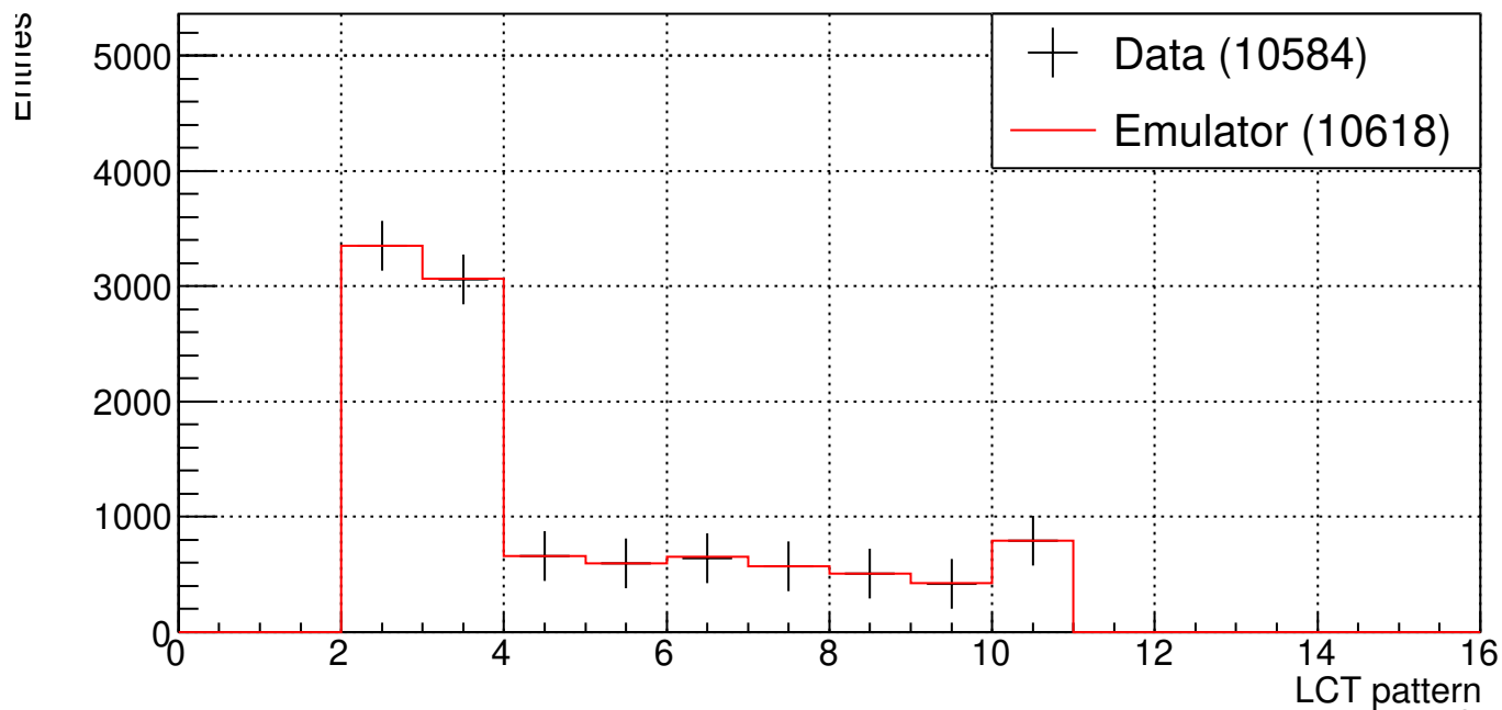
ME21 LCT pattern (B904 Cosmic Run 211105_132717)
