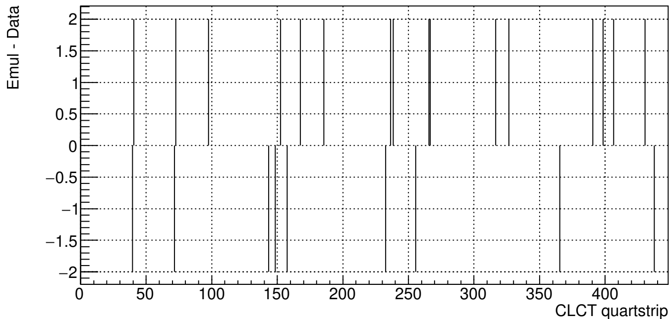
ME11 CLCT quartstrip (B904 Cosmic Run 210701_135109)
