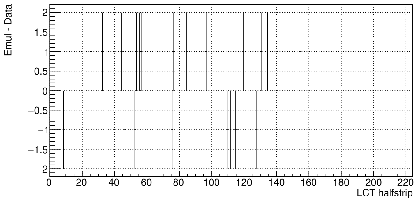
ME11 LCT halfstrip (B904 Cosmic Run 210701_135109)
