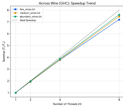
(c) Speedup of across-wires on GHC machines
