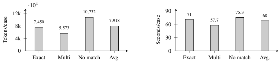
FIGURE 3: Benchmark outcome and cost summary. The resolver returns one part for sufficiently specific descriptions, preserves the expected matching set for under-specified descriptions, and returns no parts for impossible descriptions. Cost bars report mean recorded LLM tokens and mean wall-clock seconds per case.
