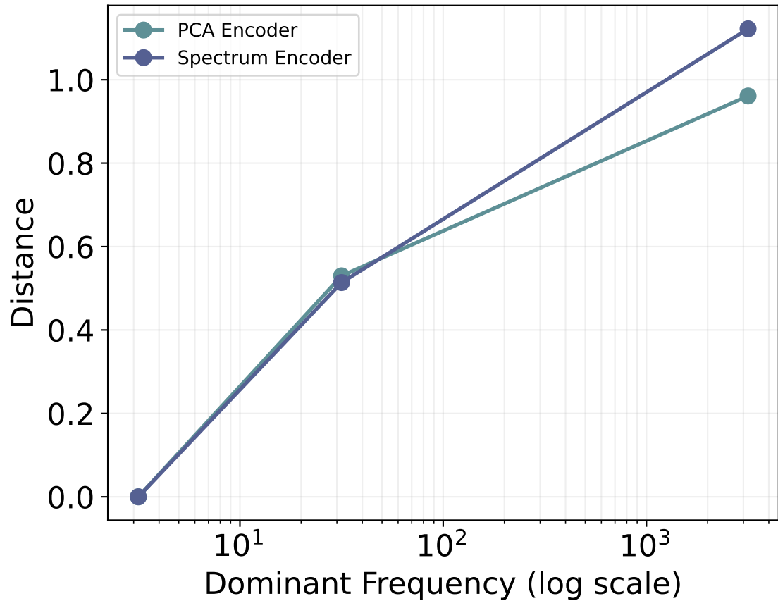
Distribution Shift (Wasserstein Distance)
