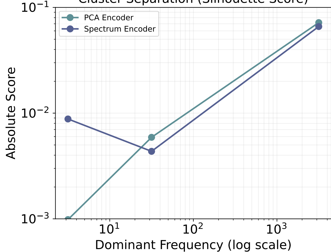
Cluster Separation (Silhouette Score)
