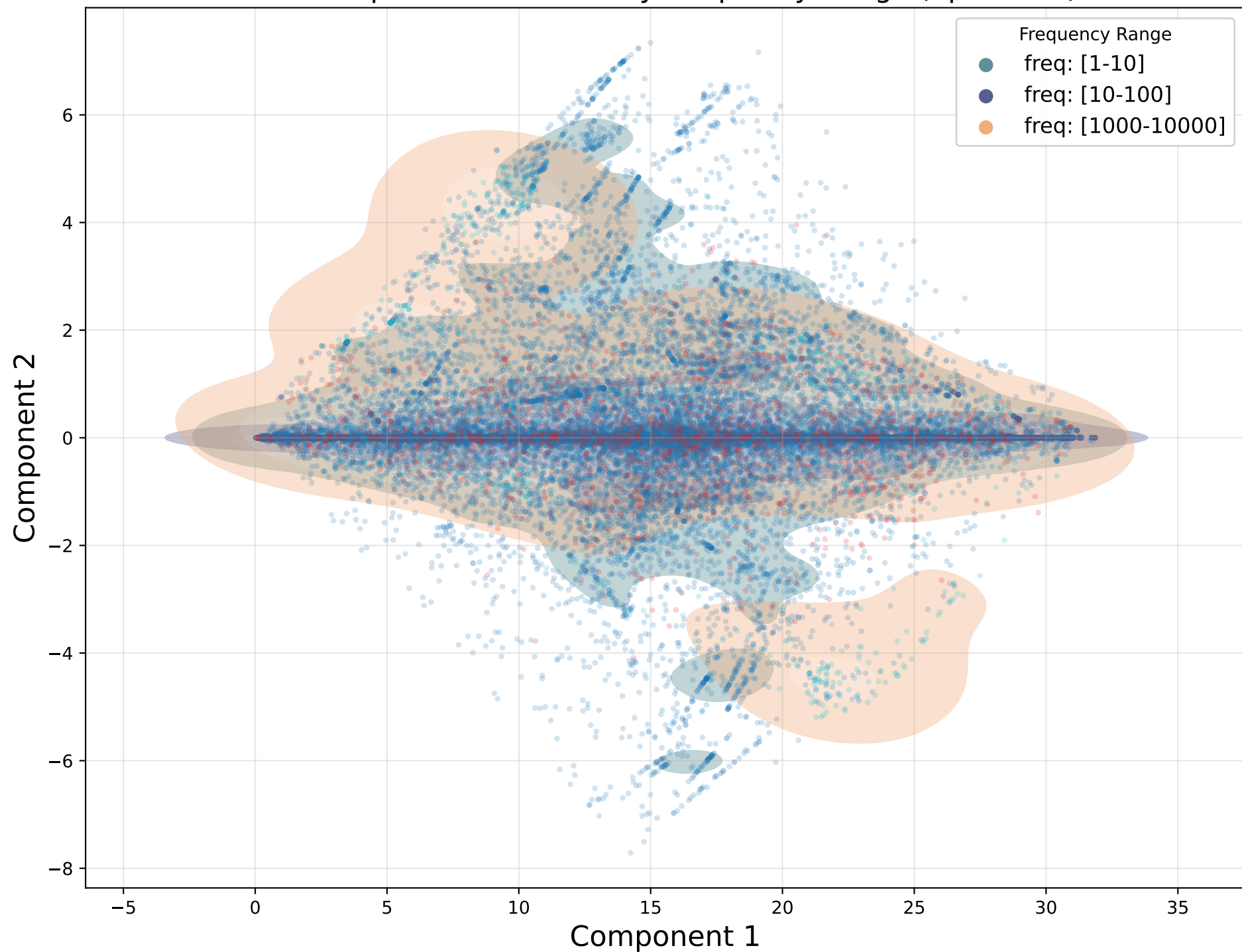
Latent Space Distribution by Frequency Range (Spectrum)
