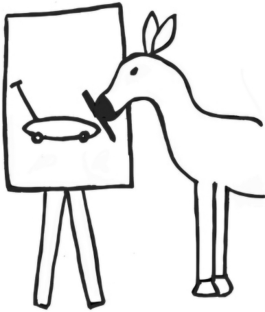
Horse-Drawn Buggy
