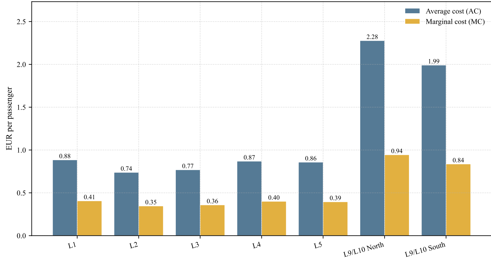
Average vs marginal cost by line, technological model (C_tec) (mean of 2023-2025; the MC/AC ratio is the basis of the Boiteux pricing rule)
