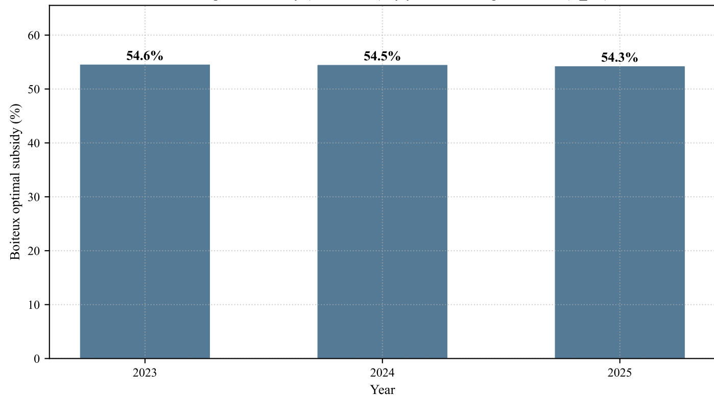
Boiteux optimal subsidy ( 1 - MC/AC ) by year, technological model (C_tec)
